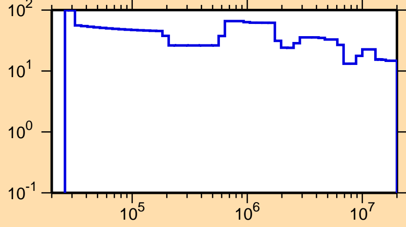
\Delta\sigma/\sigma vs. E for ^{227}\text{Ac}(n,\text{el.})
