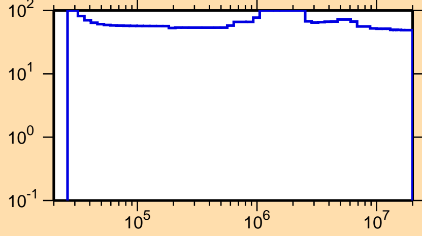
\Delta\sigma/\sigma vs. E for ^{227}\text{Ac}(n,n_1)
