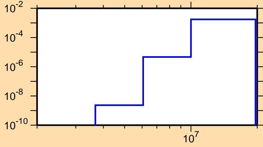
\sigma vs. E for ^{227}\text{Ac}(n,p)
