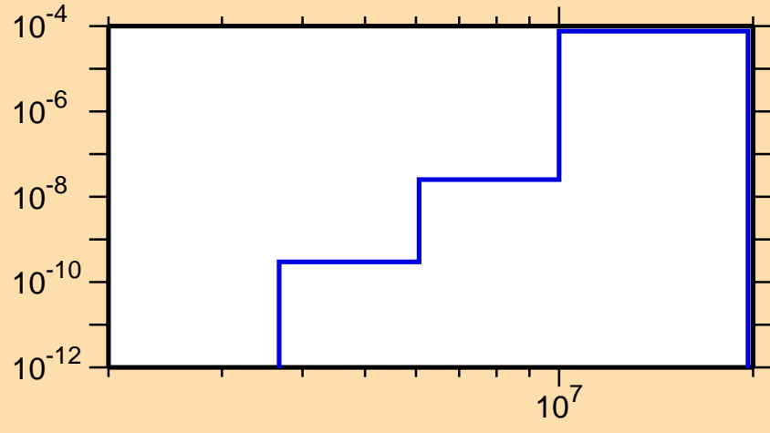
\sigma vs. E for ^{227}\text{Ac}(n,n\alpha)
