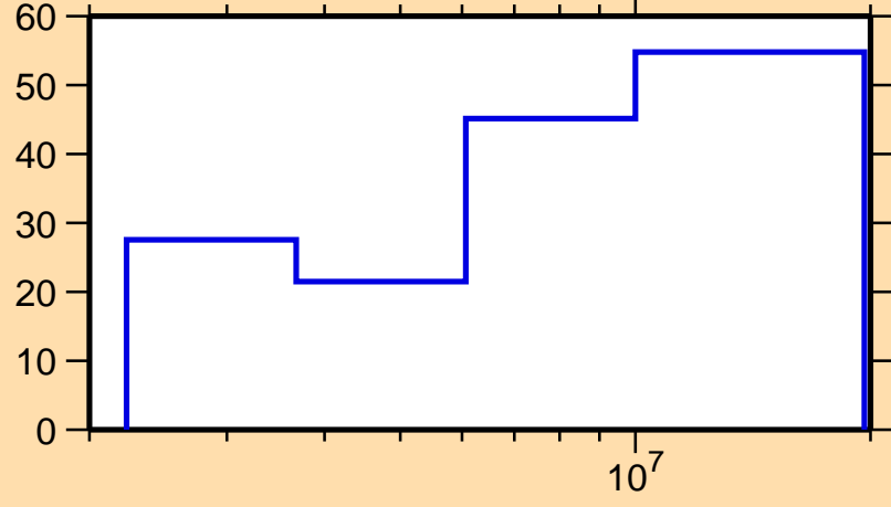
\Delta\sigma/\sigma vs. E for ^{227}\text{Ac}(n,n\text{cont.})
