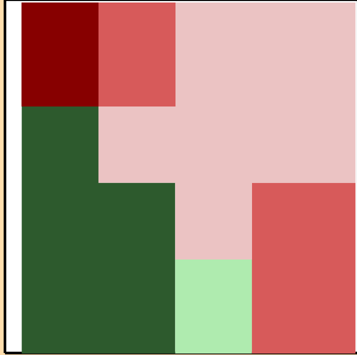
\Delta\sigma/\sigma vs. E for ^{227}\text{Ac}(n,p)
