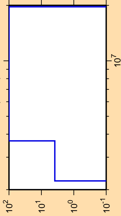
\Delta\sigma/\sigma vs. E for ^{227}\text{Ac}(n,n\alpha)
