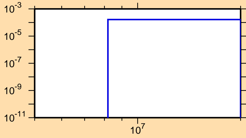
\sigma vs. E for ^{227}\text{Ac}(n,np)
