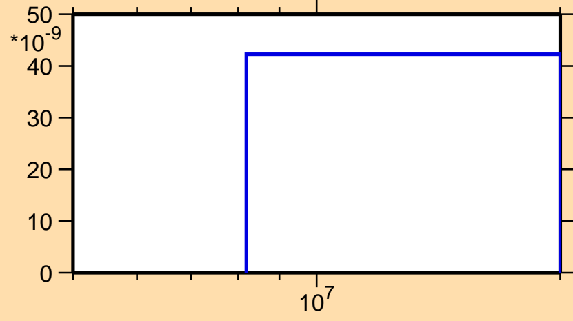
\sigma vs. E for ^{227}\text{Ac}(n,\text{nd})
