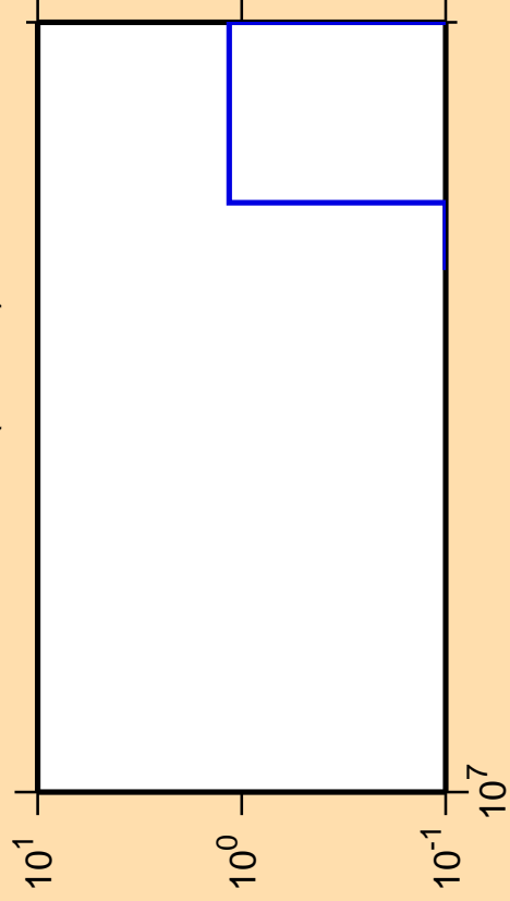
\Delta\sigma/\sigma vs. E for ^{228}\text{Ac}(\text{mt } 42)
