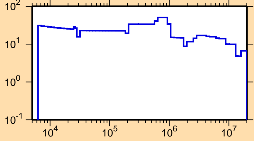
\Delta\sigma/\sigma vs. E for ^{228}\text{Ac}(n,\text{tot.})
