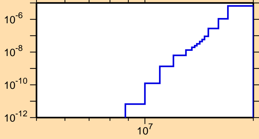
\sigma vs. E for ^{228}\text{Ac}(n,2n\alpha)
