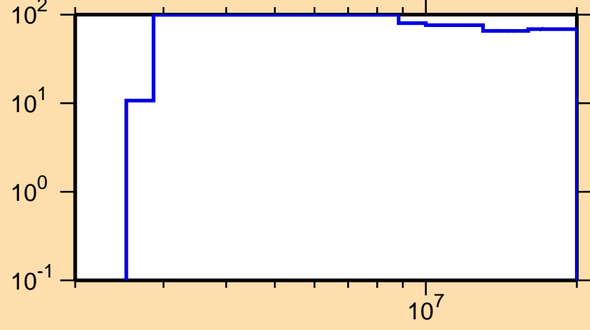
\Delta\sigma/\sigma vs. E for ^{228}\text{Ac}(n,p)
