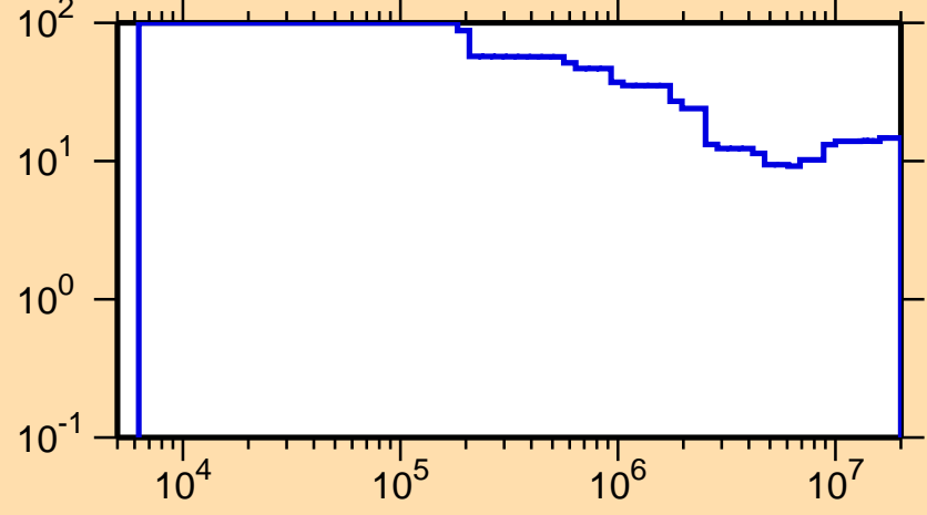
\Delta\sigma/\sigma vs. E for ^{228}\text{Ac}(n,\text{nonel.})
