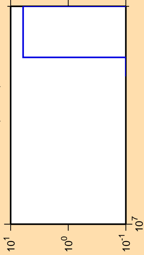
\Delta\sigma/\sigma vs. E for ^{228}\text{Ac} (mt 11)
