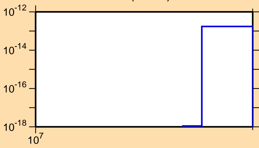
\sigma vs. E for ^{228}\text{Ac}(\text{mt } 42)
