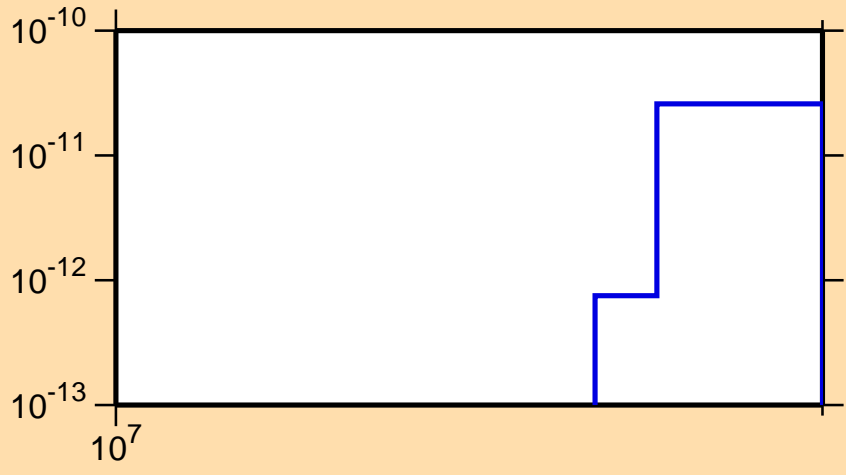
\sigma vs. E for ^{228}\text{Ac}(n,\text{He3})
