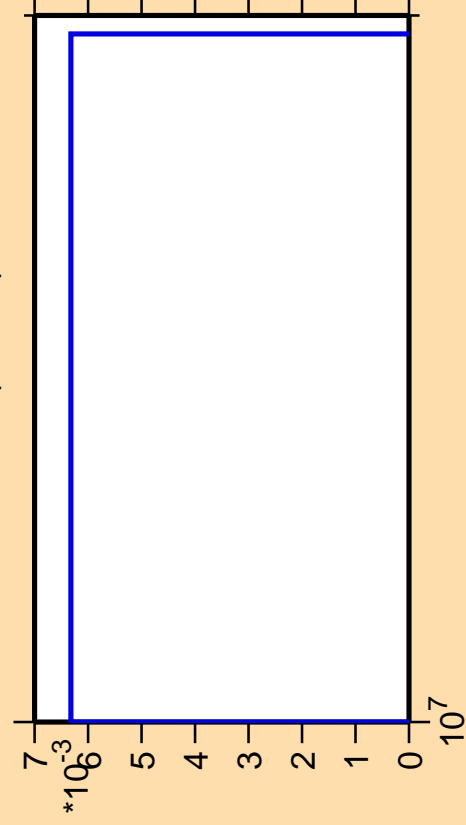
\Delta\sigma/\sigma vs. E for ^{228}\text{Ac} (mt 42)
