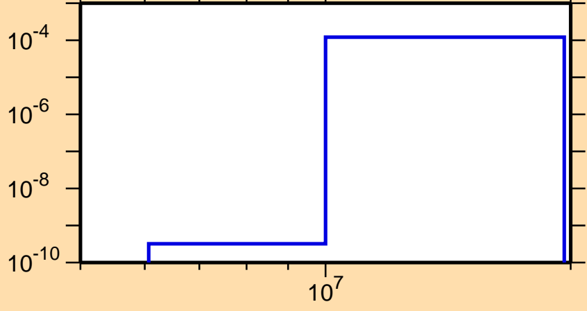
\sigma vs. E for ^{228}\text{Ac}(n,t)
