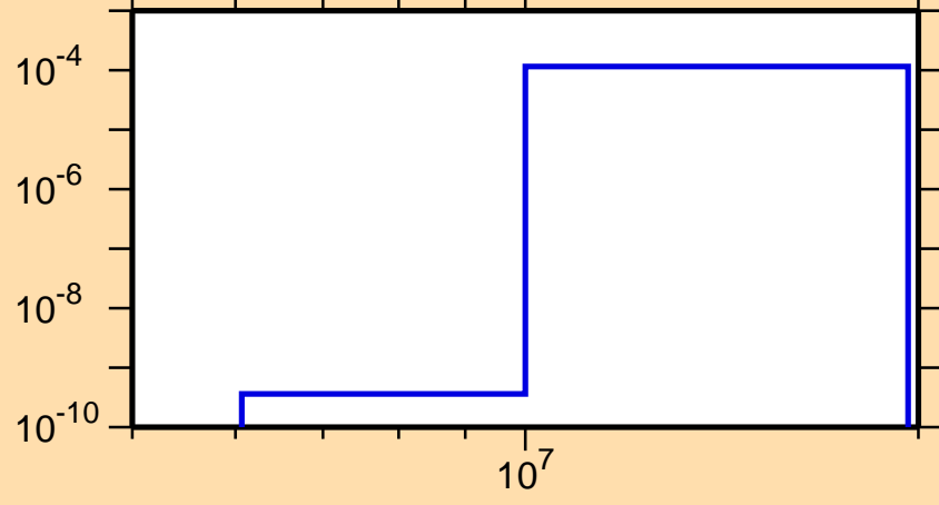
\sigma vs. E for ^{229}\text{Ac}(n,d)
