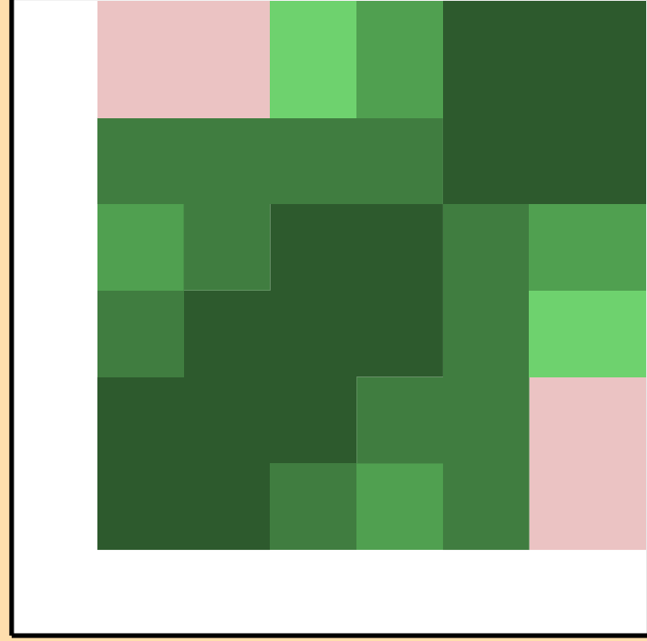
\sigma vs. E for ^{229}\text{Ac}(n,n\text{cont.})
