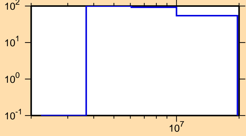
\Delta\sigma/\sigma vs. E for ^{229}\text{Ac}(n,p)
