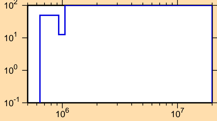
\Delta\sigma/\sigma vs. E for ^{230}\text{Ac}(n,f)
