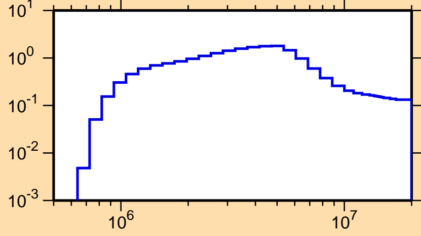
\sigma vs. E for ^{230}\text{Ac}(n,n\text{cont.})
