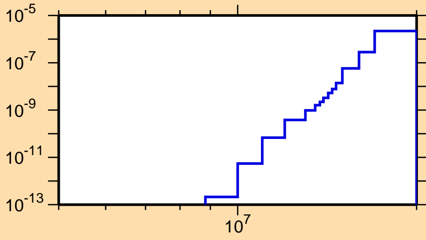
\sigma vs. E for ^{230}\text{Ac}(n,2n\alpha)
