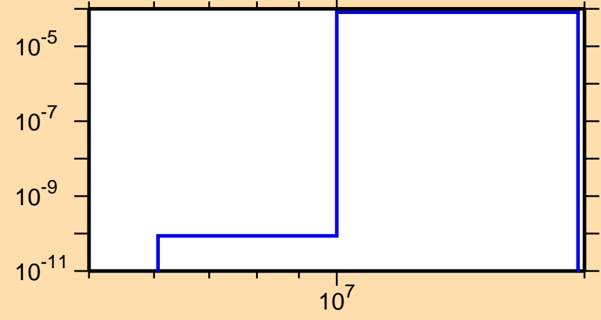
\sigma vs. E for ^{230}\text{Ac}(n,t)
