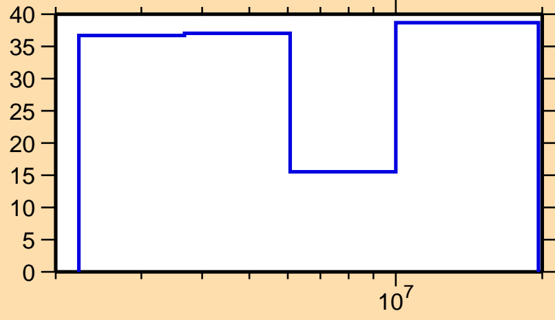
\Delta\sigma/\sigma vs. E for ^{230}\text{Ac}(n,ncont.)
