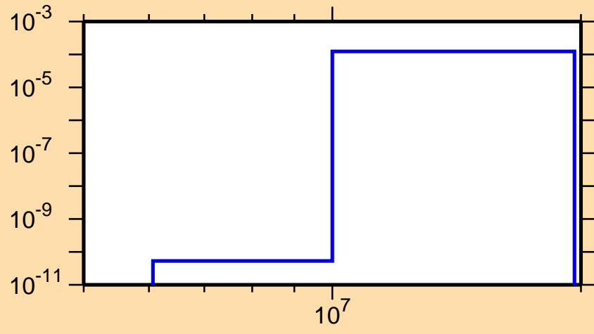
\sigma vs. E for ^{230}\text{Ac}(n,d)
