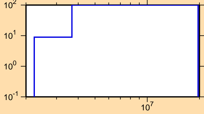
\Delta\sigma/\sigma vs. E for ^{230}\text{Ac}(n,p)
