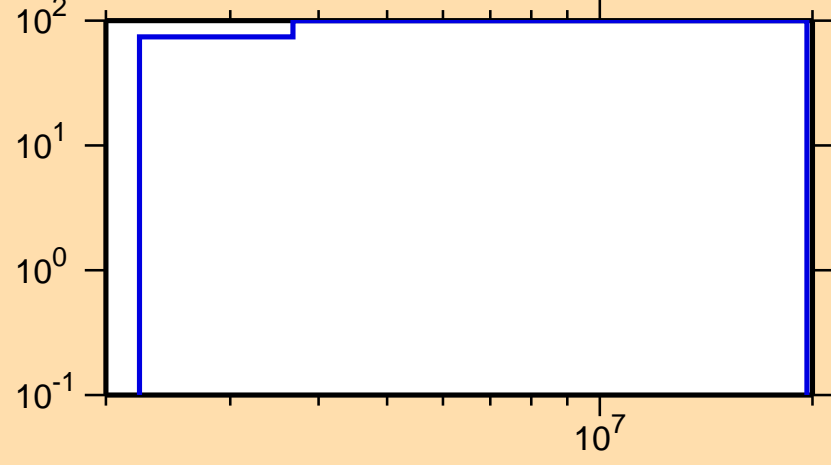
\Delta\sigma/\sigma vs. E for ^{230}\text{Ac}(n,\gamma)
