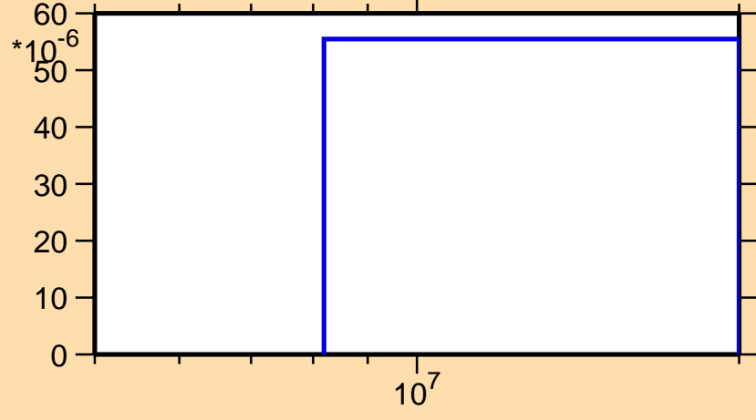
\sigma vs. E for ^{230}\text{Ac}(n,np)
