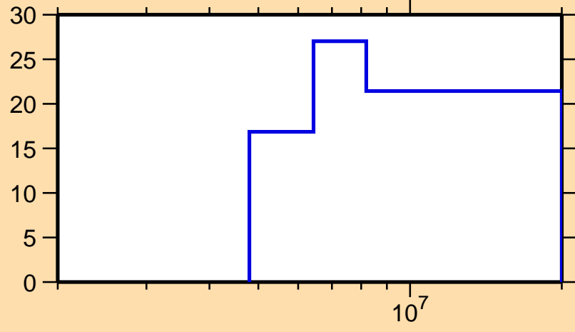
\Delta\sigma/\sigma vs. E for ^{230}\text{Ac}(n,2n)
