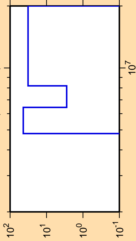
\Delta\sigma/\sigma vs. E for ^{230}\text{Ac}(n,n\text{cont.})
