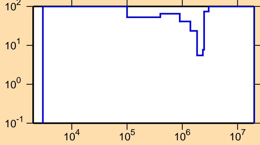
\Delta\sigma/\sigma vs. E for ^{230}\text{Ac}(n,n_1)
