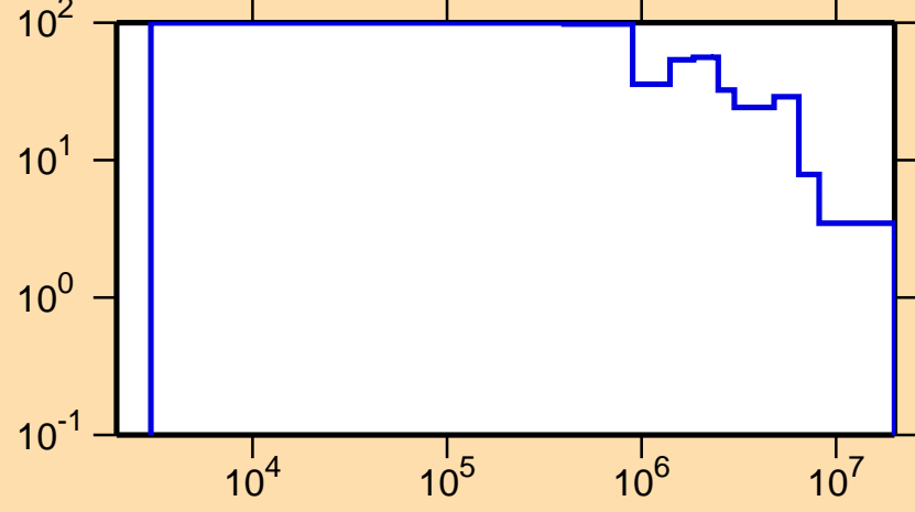
\Delta\sigma/\sigma vs. E for ^{230}\text{Ac}(n,\text{inel.})
