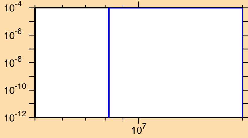
\sigma vs. E for ^{230}\text{Ac}(n,d)
