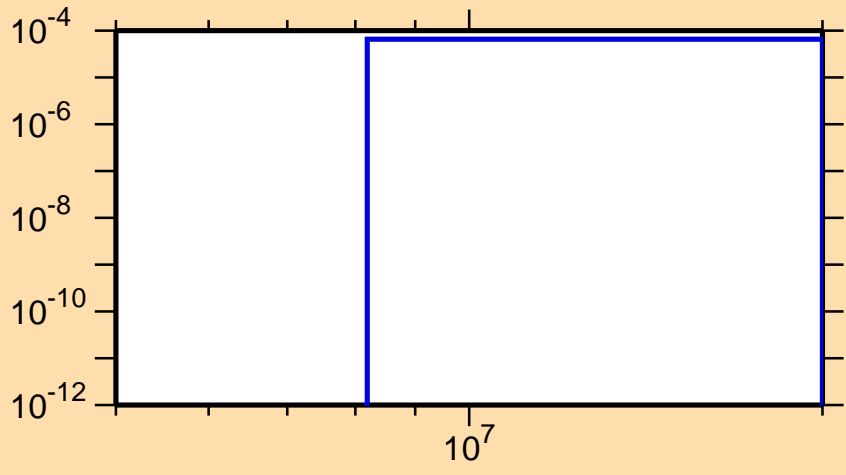
\sigma vs. E for ^{230}\text{Ac}(n,t)
