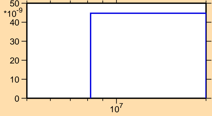
\sigma vs. E for ^{230}\text{Ac}(n,2np)
