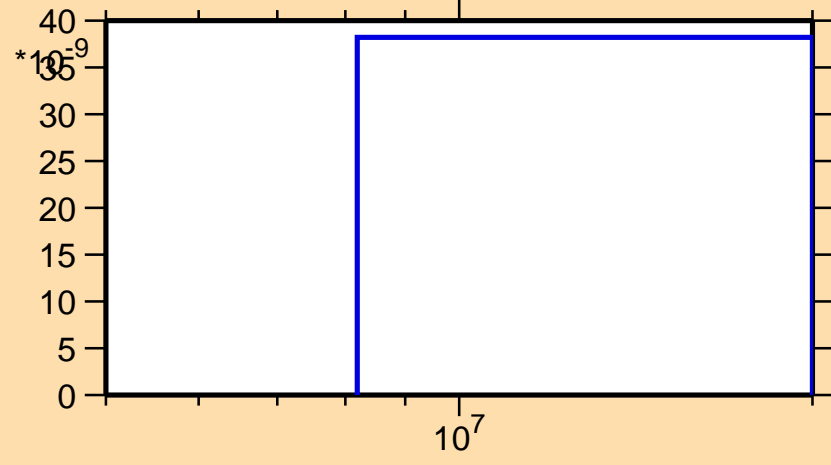
\sigma vs. E for ^{230}\text{Ac}(n,2n\alpha)
