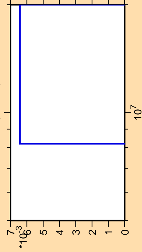
\Delta\sigma/\sigma vs. E for ^{230}\text{Ac} (mt 11)
