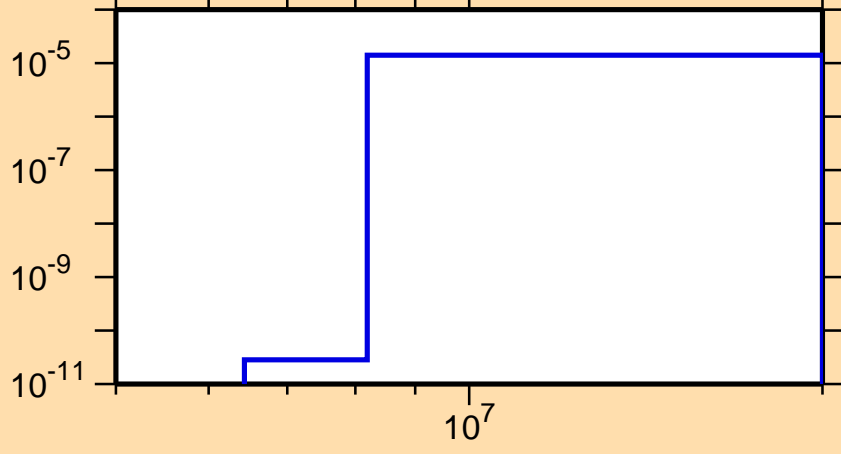
\sigma vs. E for ^{230}\text{Ac}(n,n\alpha)
