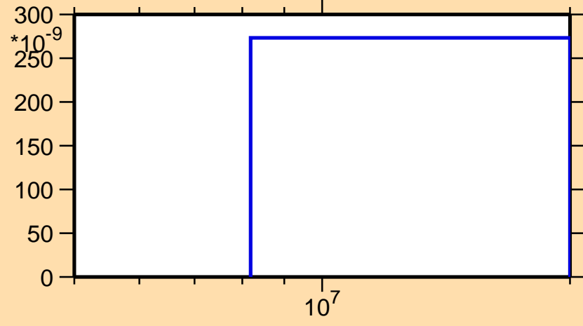
\sigma vs. E for ^{230}\text{Ac}(n,\text{nd})
