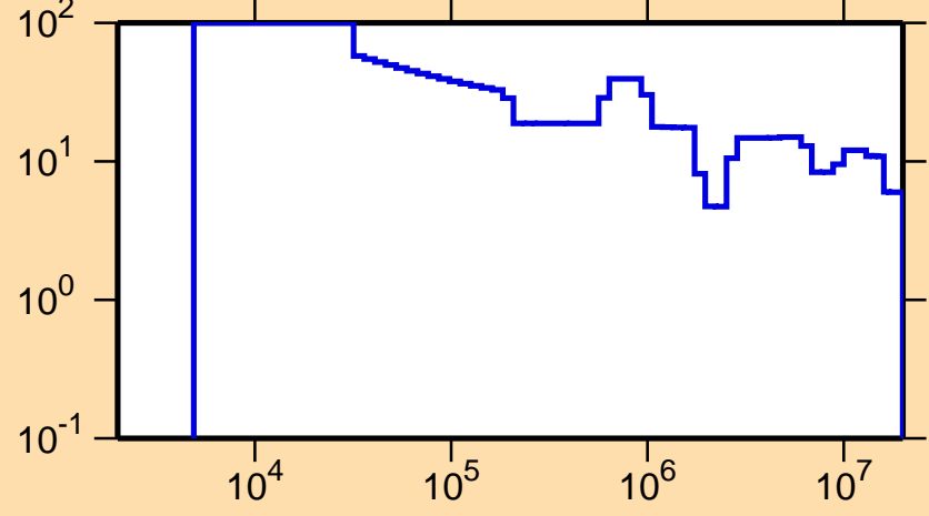
\Delta\sigma/\sigma vs. E for ^{231}\text{Ac}(n,\text{tot.})
