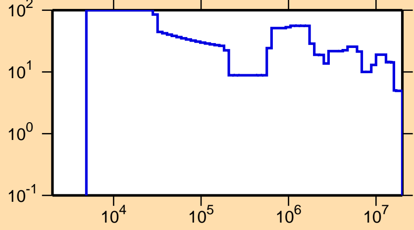
\Delta\sigma/\sigma vs. E for ^{231}\text{Ac}(n,\text{el.})
