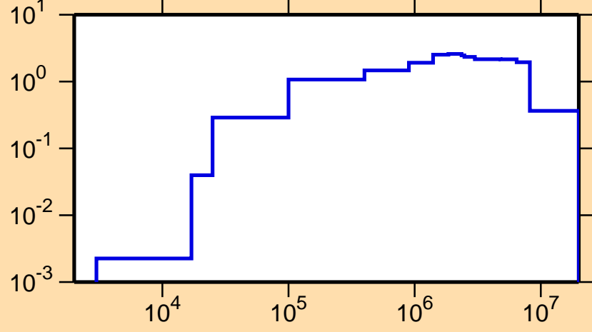
\sigma vs. E for ^{231}\text{Ac}(n,\text{inel.})
