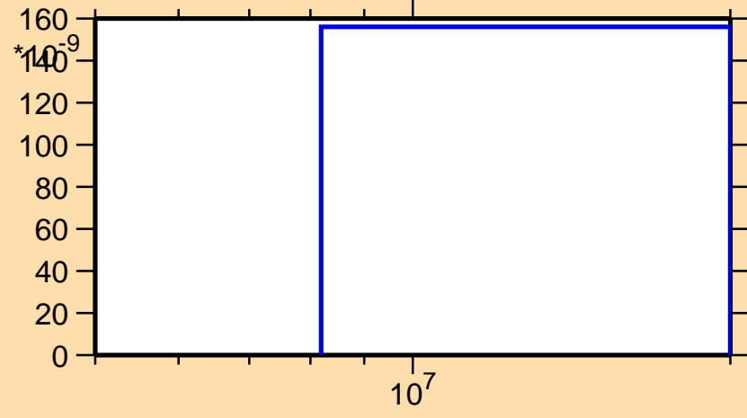
\sigma vs. E for ^{231}\text{Ac}(n,nt)
