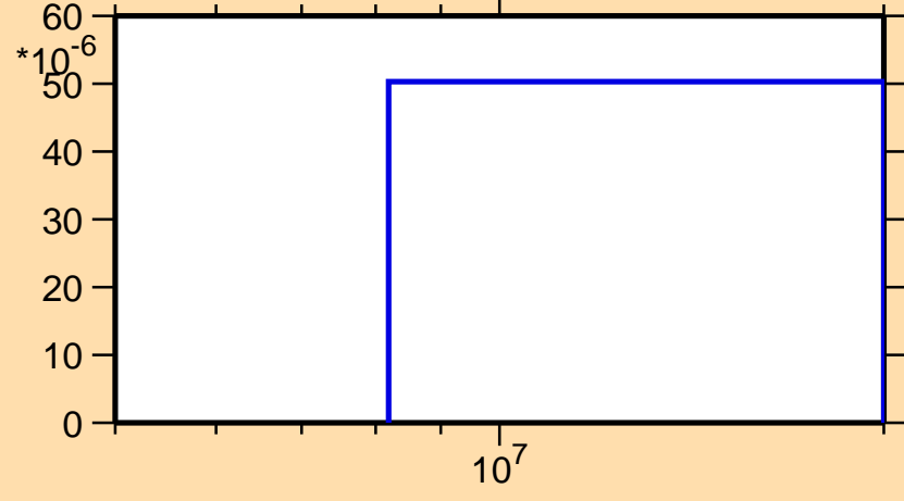
\sigma vs. E for ^{231}\text{Ac}(n,np)
