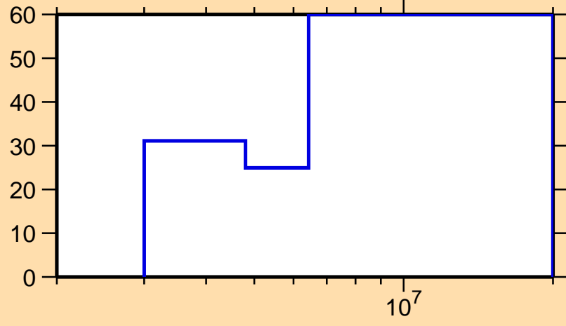
\Delta\sigma/\sigma vs. E for ^{231}\text{Ac}(n,ncont.)
