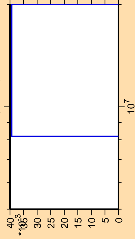
\Delta\sigma/\sigma vs. E for ^{231}\text{Ac} (mt 11)
