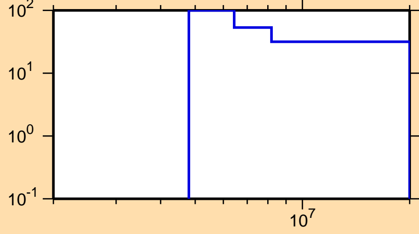
\Delta\sigma/\sigma vs. E for ^{231}\text{Ac}(n,2n)
