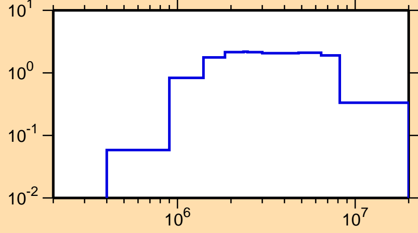
\sigma vs. E for ^{231}\text{Ac}(n,n\text{cont.})
