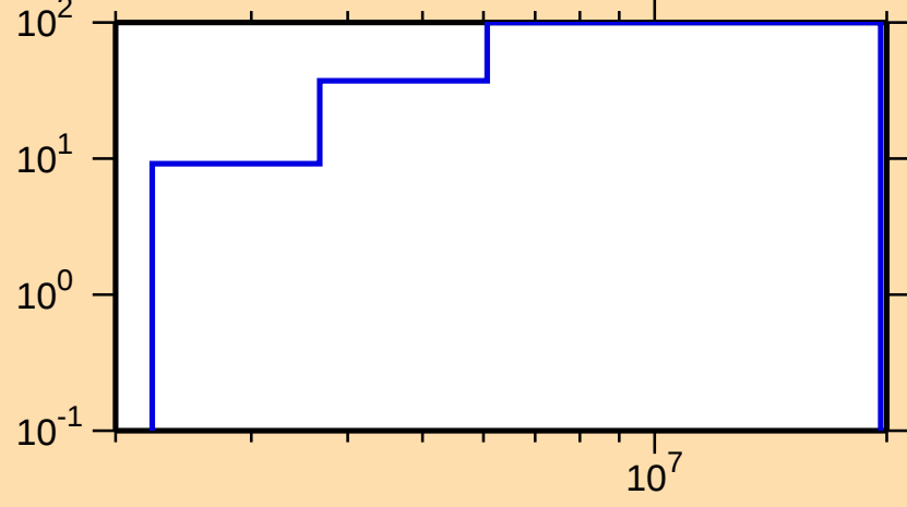
\Delta\sigma/\sigma vs. E for ^{232}\text{Ac}(n,\text{inel.})
