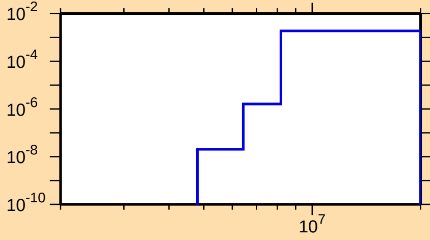
\sigma vs. E for ^{232}\text{Ac}(n,p)
