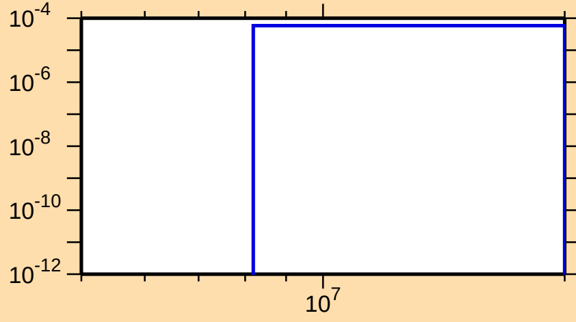
\sigma vs. E for ^{232}\text{Ac}(n,d)
