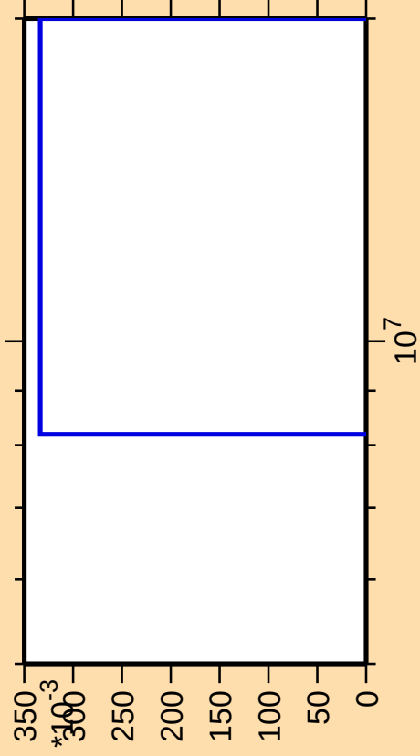
\Delta\sigma/\sigma vs. E for ^{232}\text{Ac}(n,3n\alpha)
