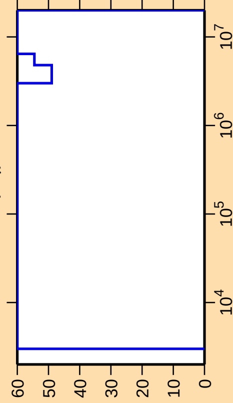
\Delta\sigma/\sigma vs. E for ^{232}\text{Ac}(n,\gamma)
