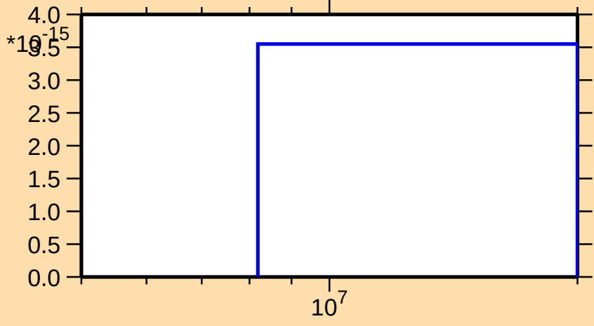
\sigma vs. E for ^{232}\text{Ac}(\text{mt 11})
