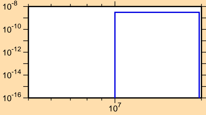
\sigma vs. E for ^{234}\text{Ac}(n,2n\alpha)
