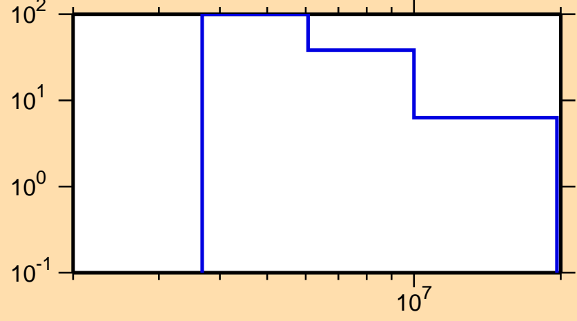
\Delta\sigma/\sigma vs. E for ^{234}\text{Ac}(n,p)
