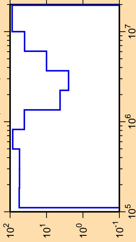
\Delta\sigma/\sigma vs. E for ^{234}\text{Ac}(n,\text{inel.})
