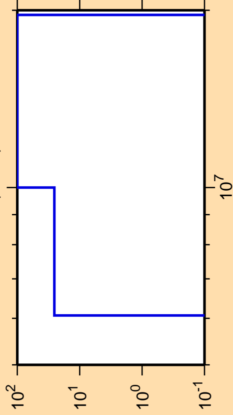
\Delta\sigma/\sigma vs. E for ^{234}\text{Ac}(n,n\alpha)
