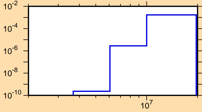
\sigma vs. E for ^{234}\text{Ac}(n,p)
