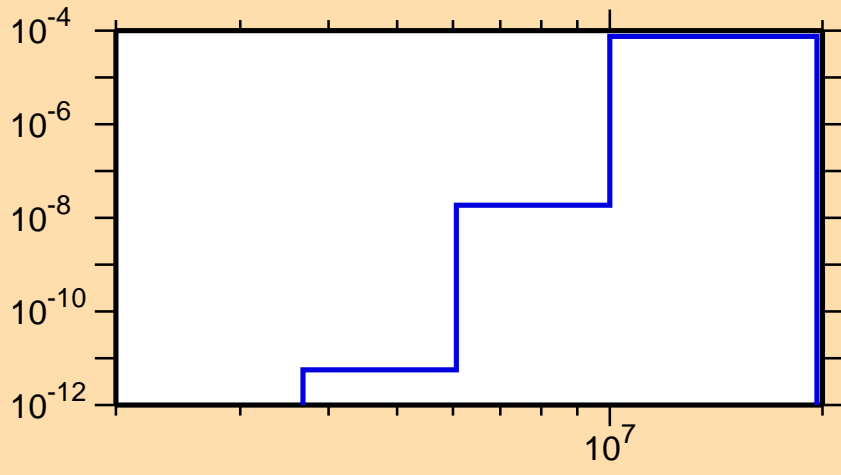
\sigma vs. E for ^{234}\text{Ac}(n,\alpha)
