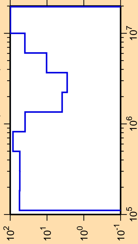
\Delta\sigma/\sigma vs. E for ^{234}\text{Ac}(n,\text{ncont.})
