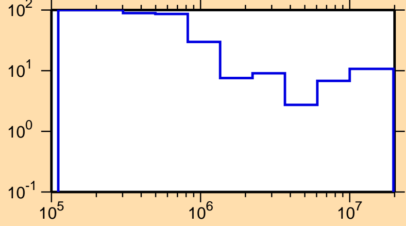
\Delta\sigma/\sigma vs. E for ^{234}\text{Ac}(n,\text{nonel.})
