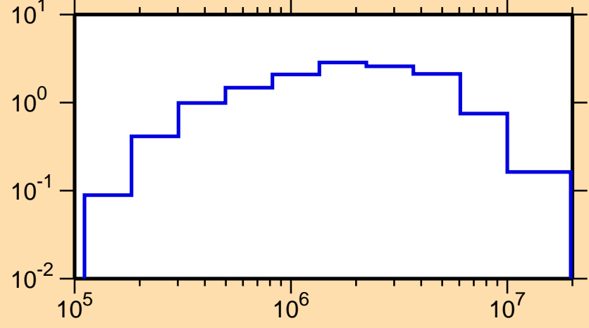
\sigma vs. E for ^{234}\text{Ac}(n,\text{inel.})
