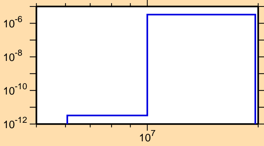
\sigma vs. E for ^{234}\text{Ac}(n,n\alpha)
