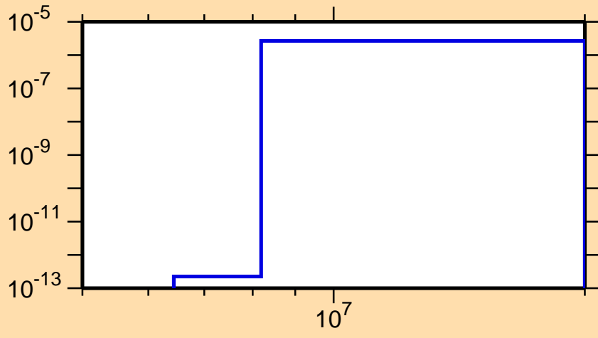
\sigma vs. E for ^{234}\text{Ac}(n,n\alpha)
