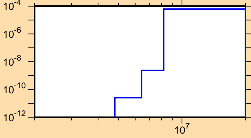
\sigma vs. E for ^{234}\text{Ac}(n,\alpha)
