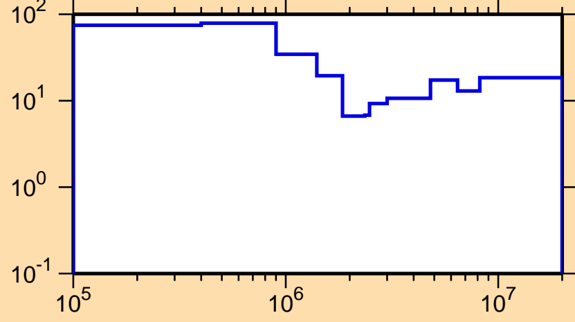
\Delta\sigma/\sigma vs. E for ^{234}\text{Ac}(n,\text{tot.})
