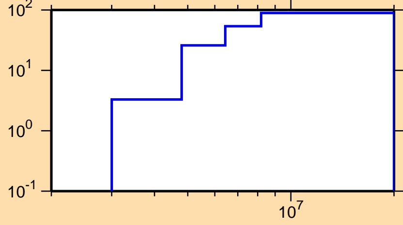
\Delta\sigma/\sigma vs. E for ^{234}\text{Ac}(n,n\text{cont.})
