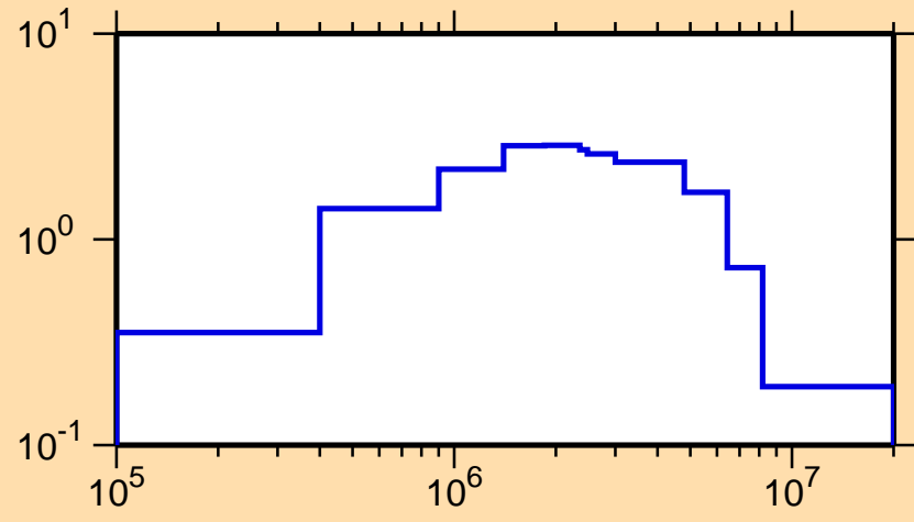
\sigma vs. E for ^{234}\text{Ac}(n,n\text{cont.})
