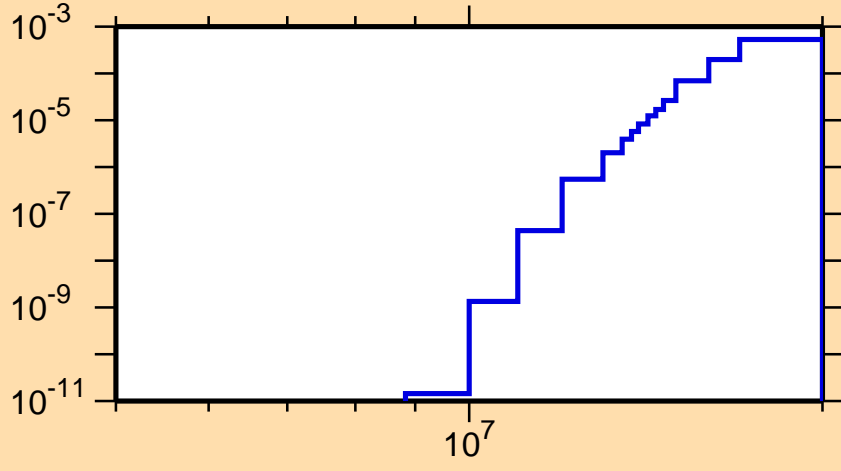
\sigma vs. E for ^{235}\text{Ac}(n,d)
