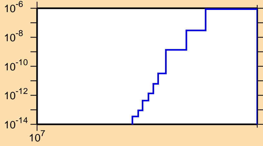
\sigma vs. E for ^{235}\text{Ac}(n,\text{nd})
