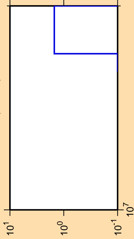
\Delta\sigma/\sigma vs. E for ^{235}\text{Ac}(n,3n\alpha)
