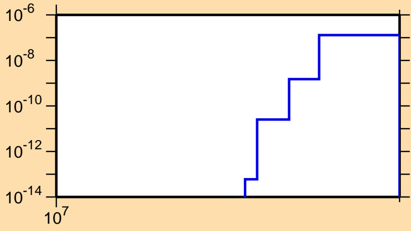
\sigma vs. E for ^{235}\text{Ac}(n,2np)
