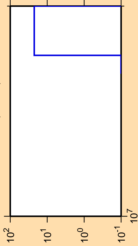
\Delta\sigma/\sigma vs. E for ^{235}\text{Ac}(\text{mt } 11)
