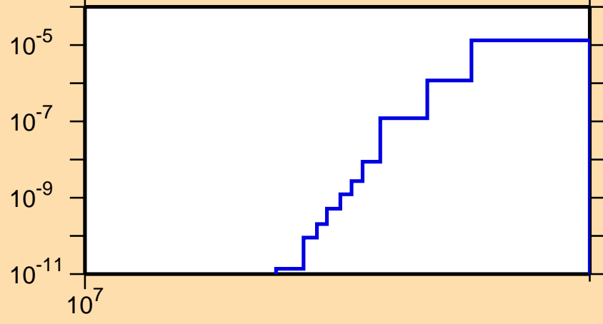
\sigma vs. E for ^{235}\text{Ac}(n,nt)
