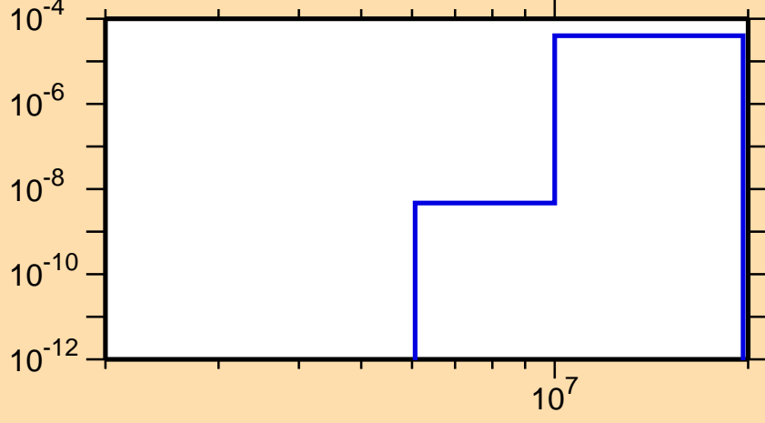
\sigma vs. E for ^{235}\text{Ac}(n,\alpha)
