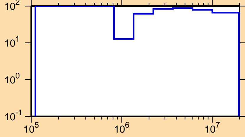
\Delta\sigma/\sigma vs. E for ^{235}\text{Ac}(n,\text{inel.})
