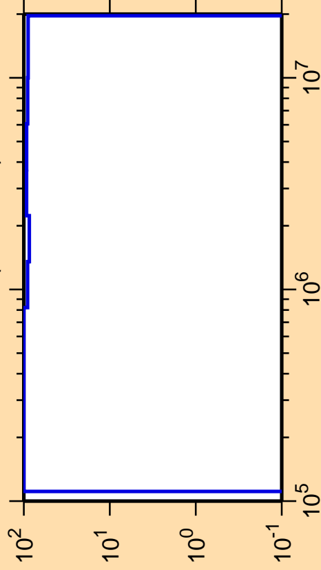
\Delta\sigma/\sigma vs. E for ^{235}\text{Ac}(n,n\text{cont.})
