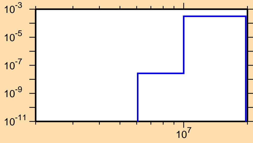
\sigma vs. E for ^{235}\text{Ac}(n,p)
