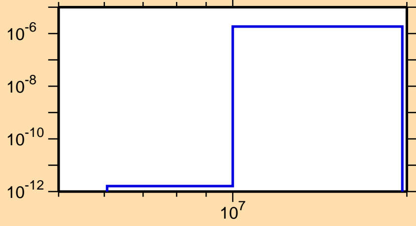
\sigma vs. E for ^{235}\text{Ac}(n,n\alpha)
