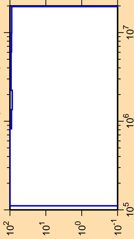
\Delta\sigma/\sigma vs. E for ^{235}\text{Ac}(n,\text{ncont.})
