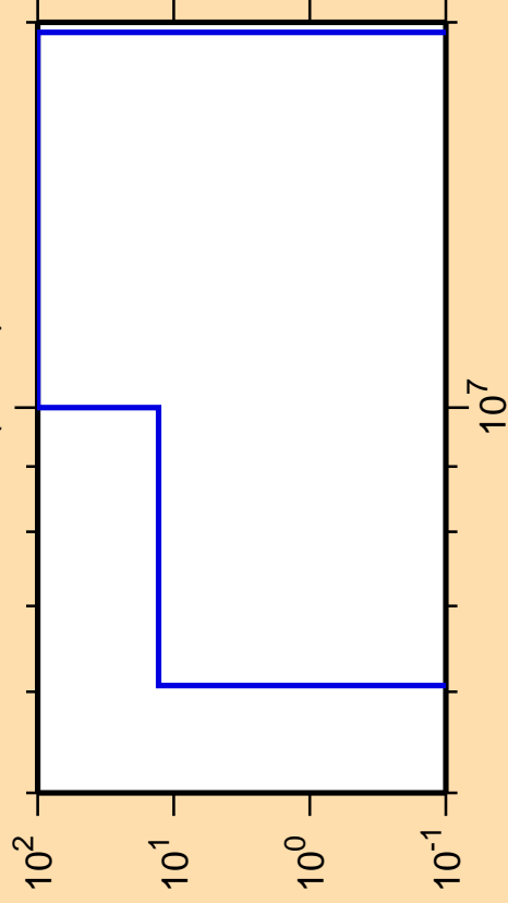
\Delta\sigma/\sigma vs. E for ^{235}\text{Ac}(n,n\alpha)
