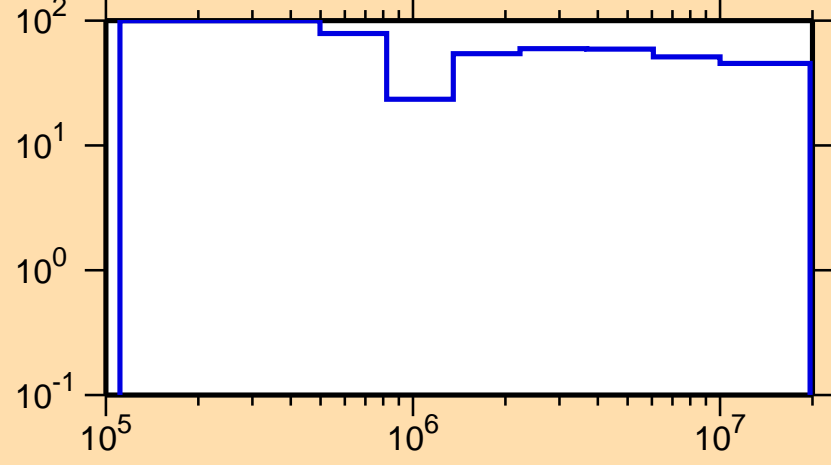
\Delta\sigma/\sigma vs. E for ^{235}\text{Ac}(n,\text{nonel.})
