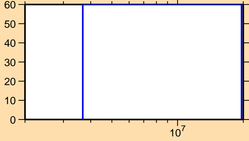
\Delta\sigma/\sigma vs. E for ^{235}\text{Ac}(n,n\text{cont.})
