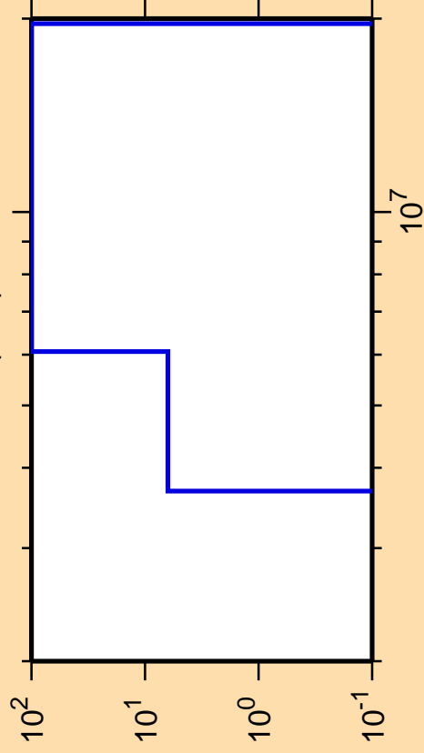
\Delta\sigma/\sigma vs. E for ^{235}\text{Ac}(n,\alpha)
