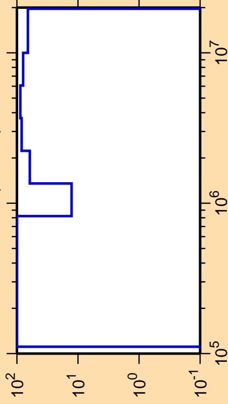
\Delta\sigma/\sigma vs. E for ^{235}\text{Ac}(n,\text{inel.})
