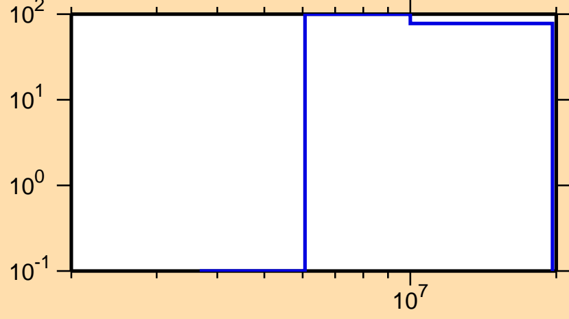
\Delta\sigma/\sigma vs. E for ^{235}\text{Ac}(n,p)
