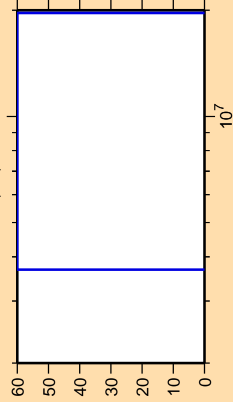
\Delta\sigma/\sigma vs. E for ^{235}\text{Ac}(n,f)
