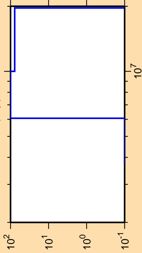
\Delta\sigma/\sigma vs. E for ^{235}\text{Ac}(n,p)
