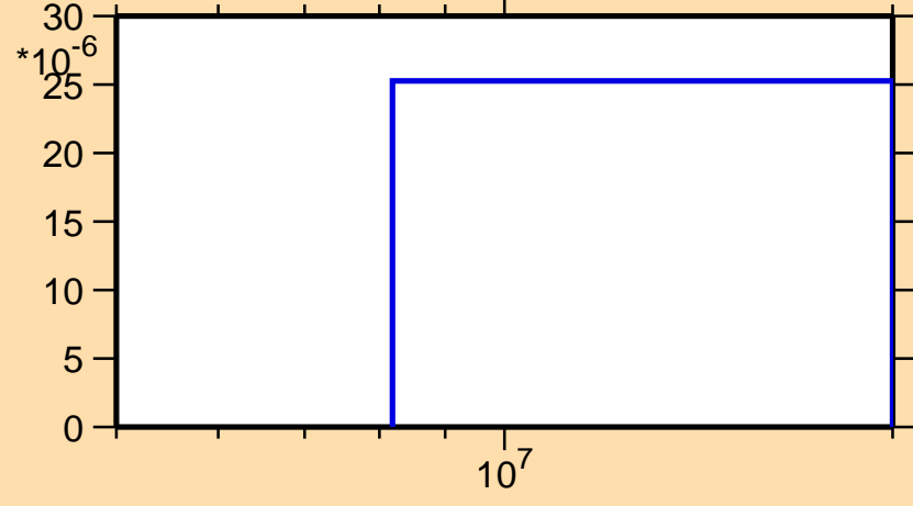
\sigma vs. E for ^{235}\text{Ac}(n,d)
