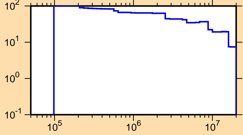
\Delta\sigma/\sigma vs. E for ^{236}\text{Ac}(n,\text{nonel.})
