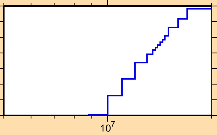
\sigma vs. E for ^{236}\text{Ac}(n,n\alpha)
