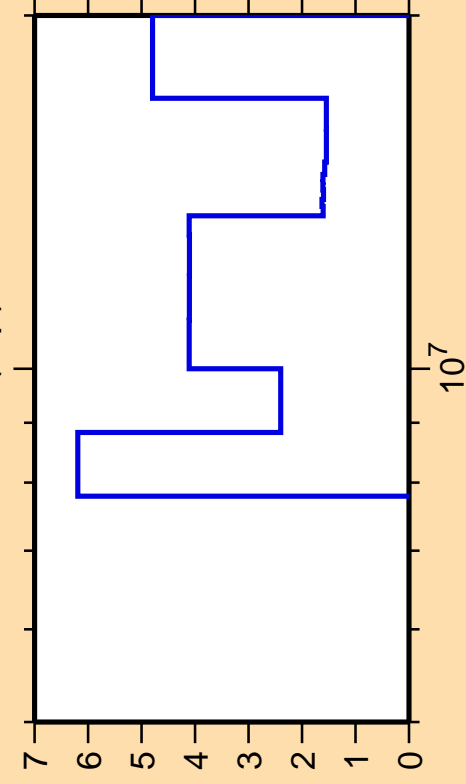
\Delta\sigma/\sigma vs. E for ^{231}\text{Am}(n,p)
