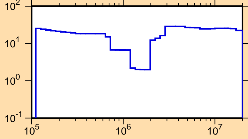
\Delta\sigma/\sigma vs. E for ^{231}\text{Am}(n,\text{nonel.})
