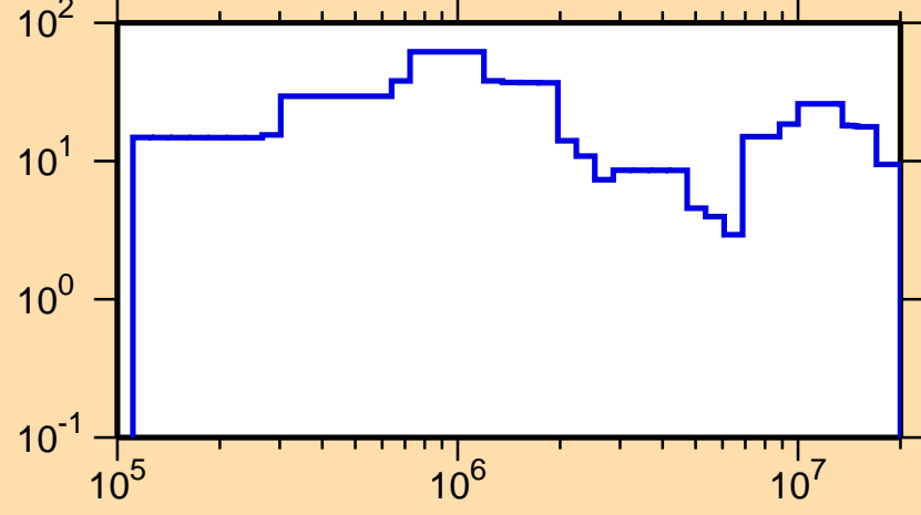
\Delta\sigma/\sigma vs. E for ^{231}\text{Am}(n,\text{el.})
