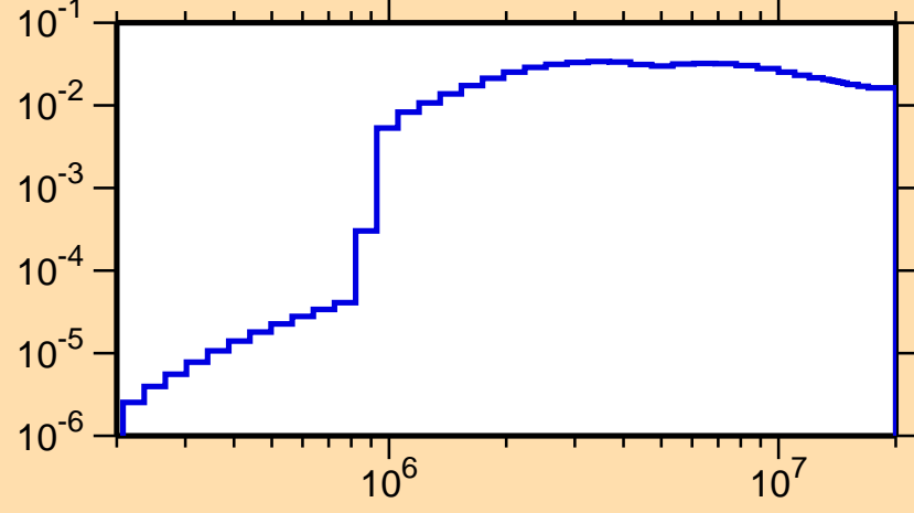
\sigma vs. E for ^{231}\text{Am}(n,n\text{cont.})
