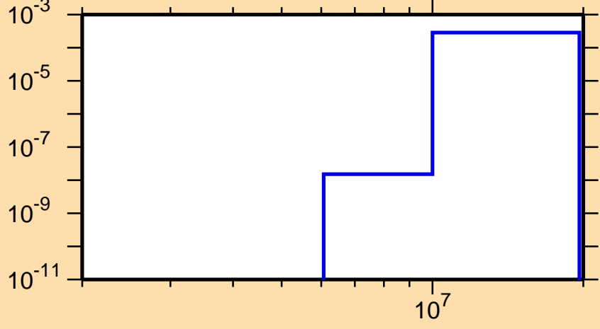
\sigma vs. E for ^{231}\text{Am}(n,np)
