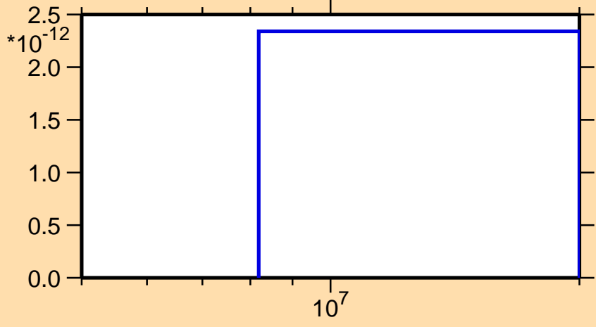
\sigma vs. E for ^{231}\text{Am} (mt 45)
