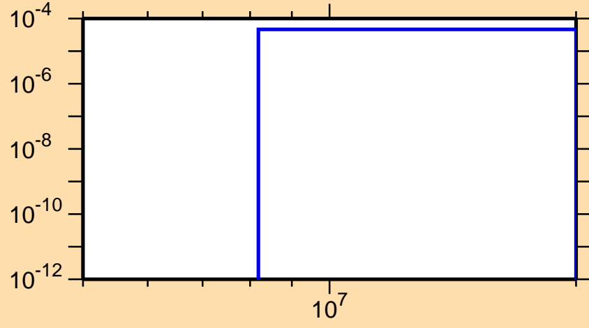
\sigma vs. E for ^{231}\text{Am}(n,t)
