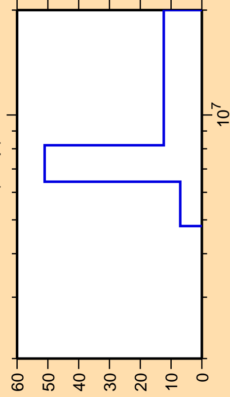
\Delta\sigma/\sigma vs. E for ^{231}\text{Am}(n,np)
