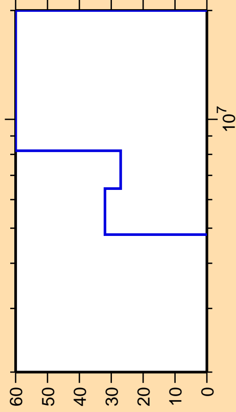
\Delta\sigma/\sigma vs. E for ^{231}\text{Am}(n,d)
