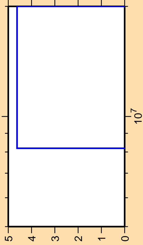
\Delta\sigma/\sigma vs. E for ^{231}\text{Am}(n,2np)
