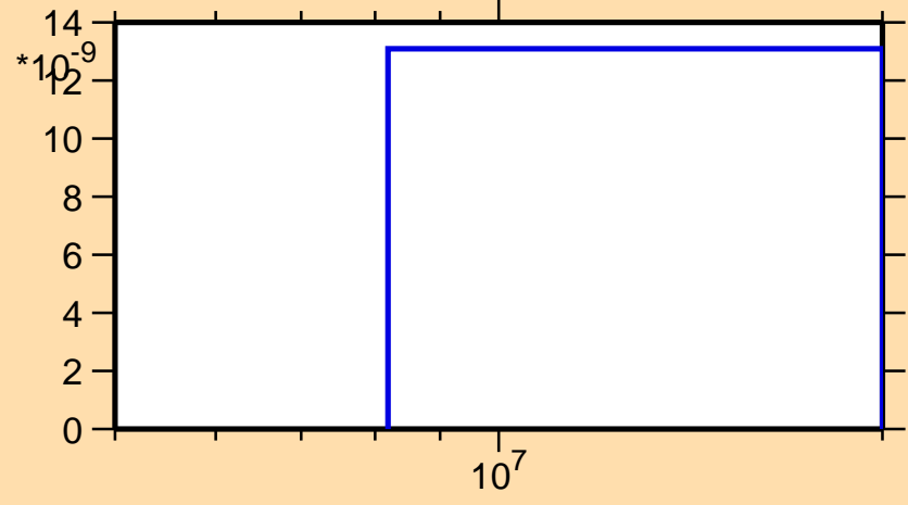
\sigma vs. E for ^{231}\text{Am}(n,\text{He3})
