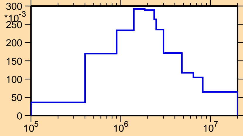
\sigma vs. E for ^{231}\text{Am}(n,\text{inel.})
