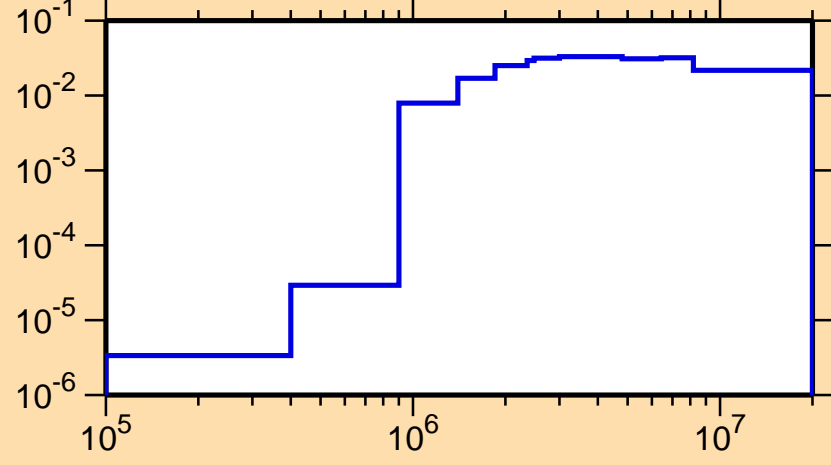
\sigma vs. E for ^{231}\text{Am}(n,n\text{cont.})
