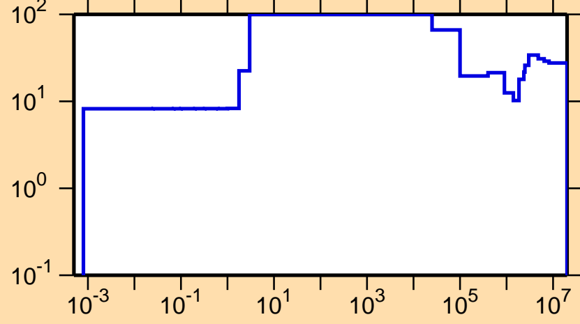
\Delta\sigma/\sigma vs. E for ^{231}\text{Am}(n, f)
