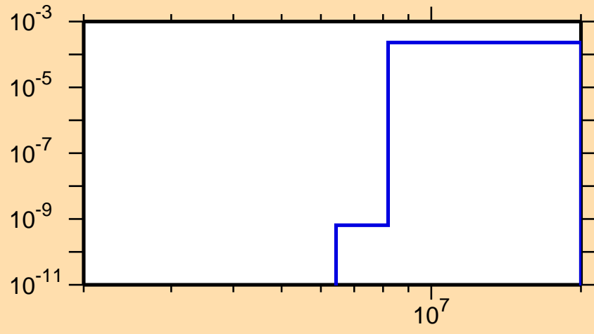
\sigma vs. E for ^{231}\text{Am}(n,np)
