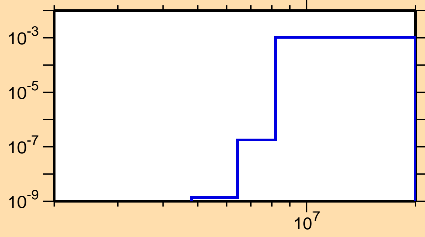
\sigma vs. E for ^{231}\text{Am}(n,d)
