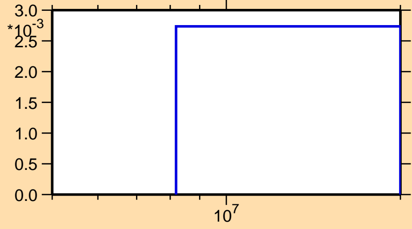
\sigma vs. E for ^{231}\text{Am}(n,2n)
