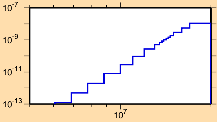
\sigma vs. E for ^{232}\text{Am}(n,p\alpha)
