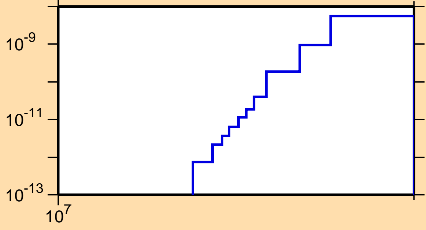
\sigma vs. E for ^{232}\text{Am}(n,nd)
