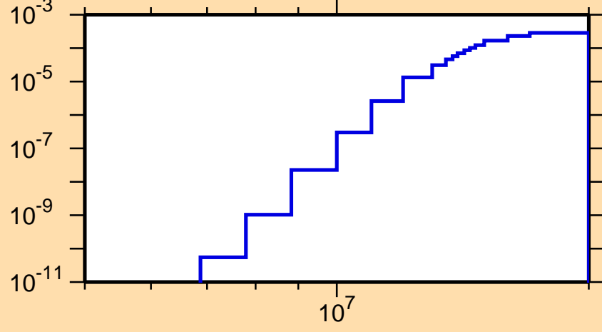
\sigma vs. E for ^{232}\text{Am}(n,t)
