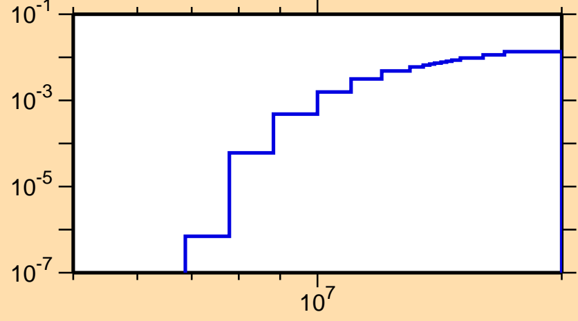
\sigma vs. E for ^{232}\text{Am}(n,2n)
