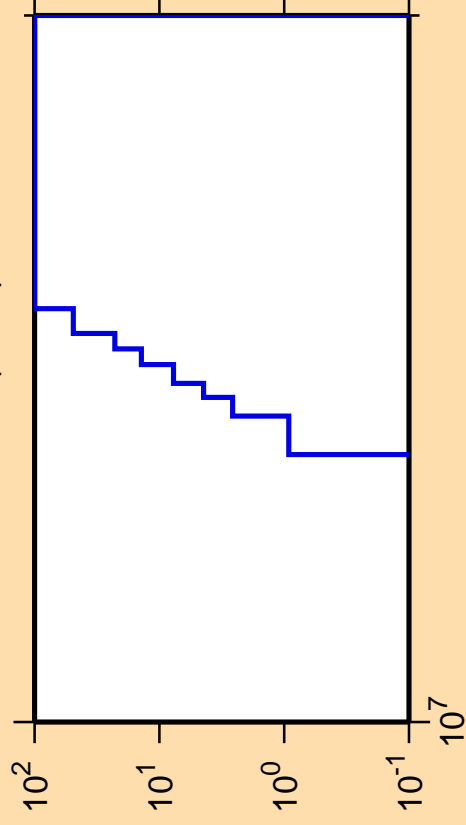
\Delta\sigma/\sigma vs. E for ^{232}\text{Am}(n,nd)
