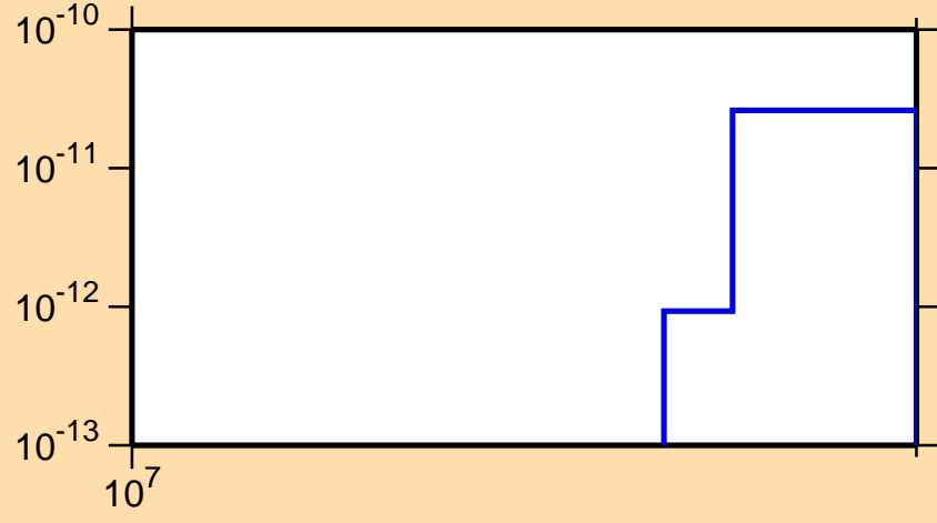
\sigma vs. E for ^{232}\text{Am} (mt 34)
