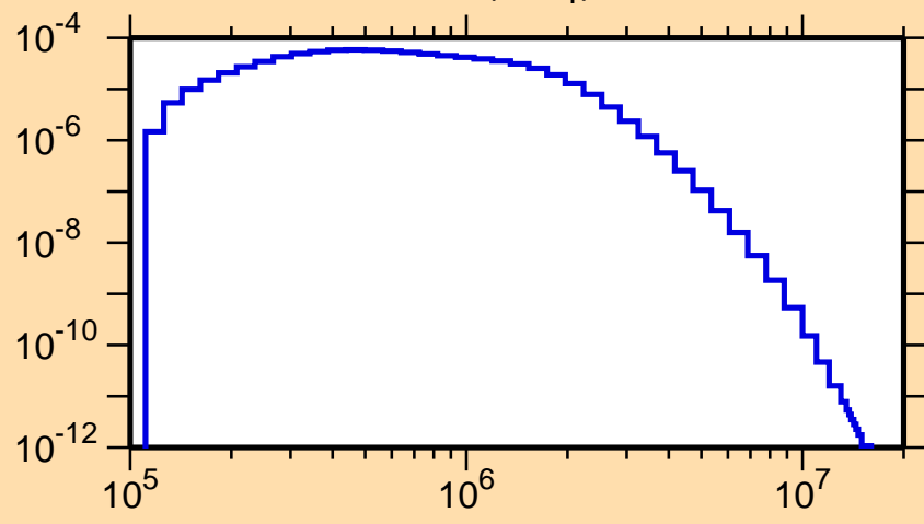
\sigma vs. E for ^{232}\text{Am}(n,n_1)
