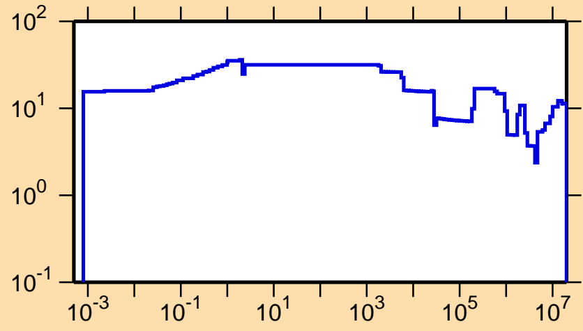
\Delta\sigma/\sigma vs. E for ^{232}\text{Am}(n,tot.)
