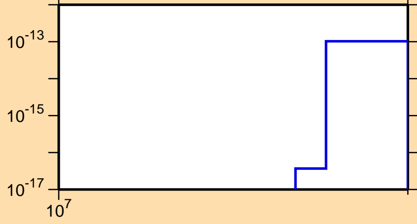
\sigma vs. E for ^{232}\text{Am}(n,3n\alpha)
