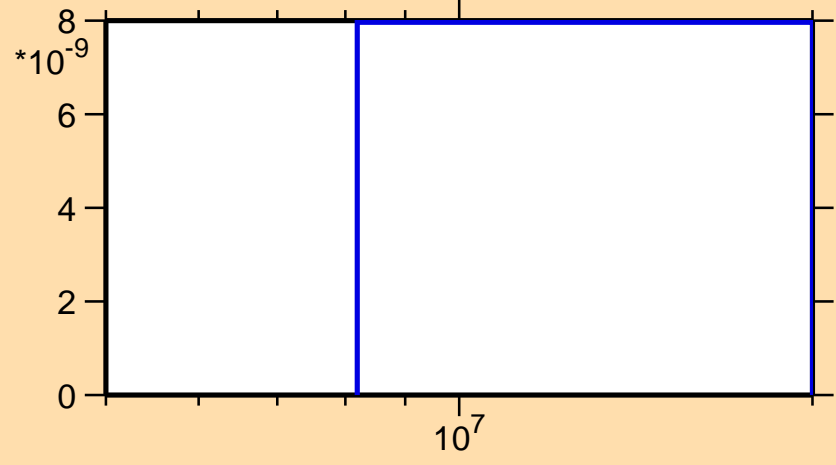
\sigma vs. E for ^{232}\text{Am}(n,3n)
