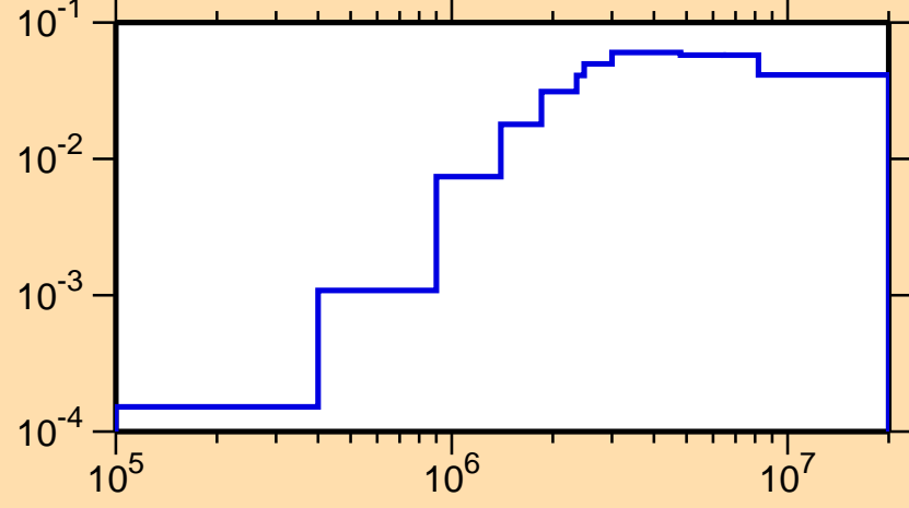
\sigma vs. E for ^{232}\text{Am}(n,\text{inel.})
