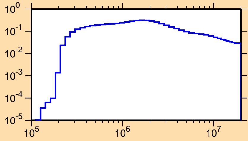
\sigma vs. E for ^{233}\text{Am}(n,n_1)
