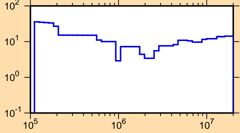
\Delta\sigma/\sigma vs. E for ^{233}\text{Am}(n,f)
