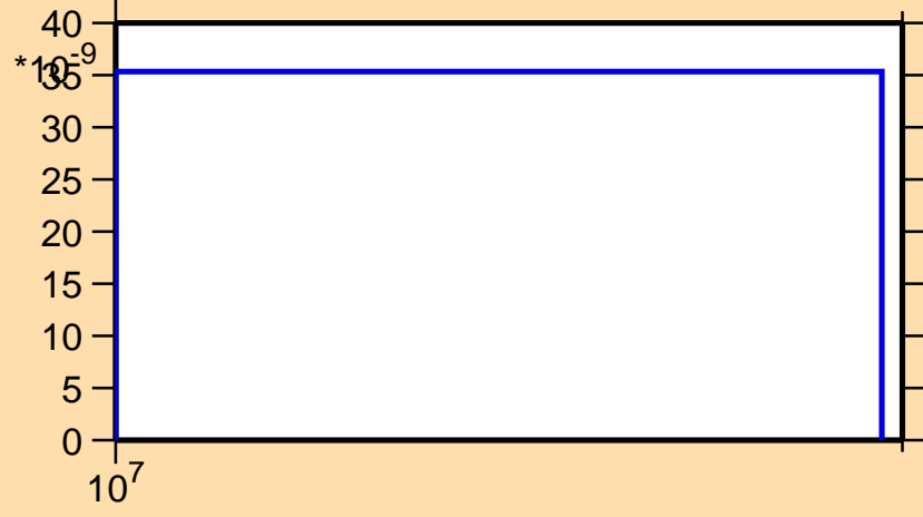
\sigma vs. E for ^{233}\text{Am}(n,3n)
