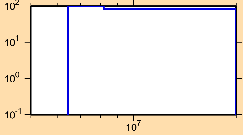
\Delta\sigma/\sigma vs. E for ^{233}\text{Am}(n,2n)
