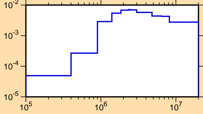
\sigma vs. E for ^{233}\text{Am}(n,n\text{cont.})
