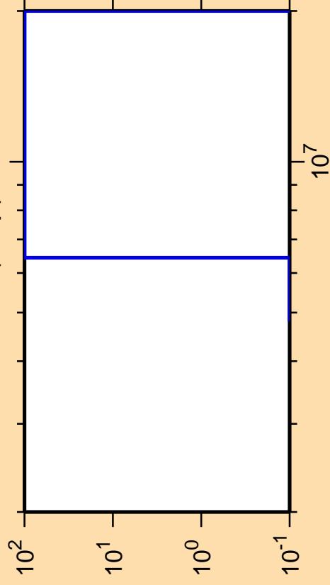
\Delta\sigma/\sigma vs. E for ^{233}\text{Am}(n,np)
