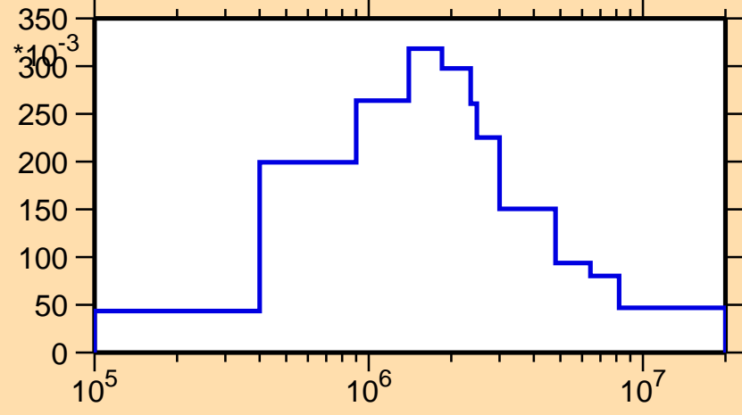
\sigma vs. E for ^{233}\text{Am}(n,\text{inel.})
