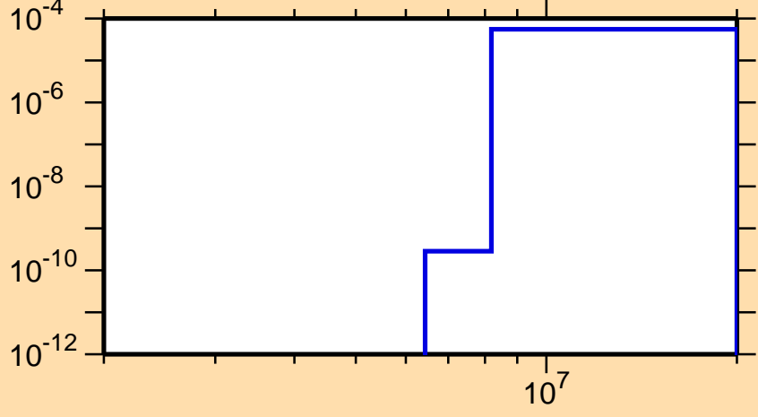
\sigma vs. E for ^{233}\text{Am}(n,np)
