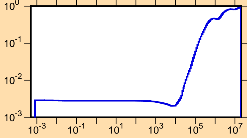
\mu vs. E for ^{234}\text{Am} (mt251)
