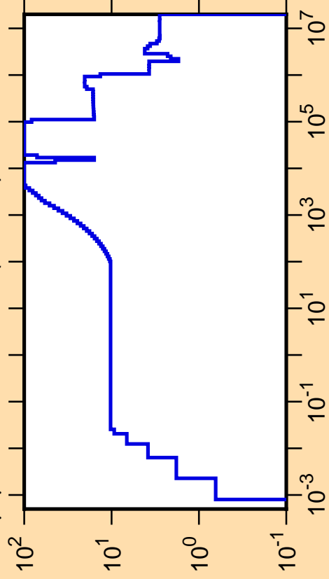
\Delta\mu/\mu vs. E for ^{234}\text{Am} (mt251)
