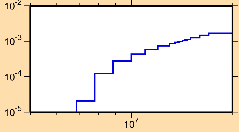
\sigma vs. E for ^{234}\text{Am}(n,2n)
