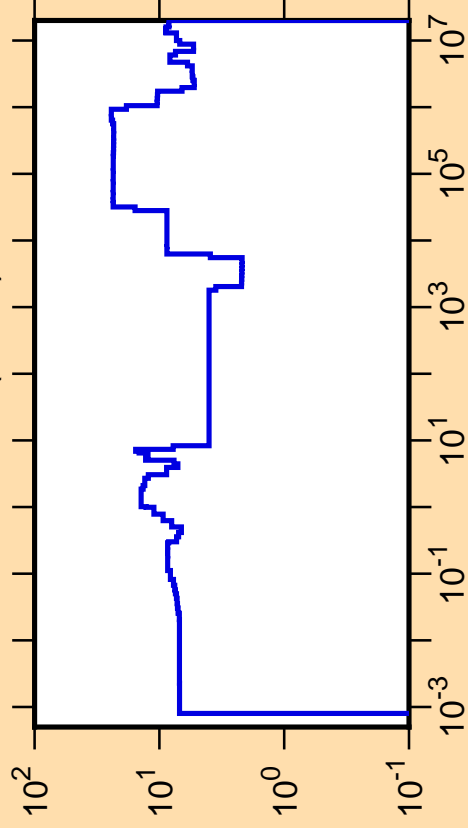
\Delta\sigma/\sigma vs. E for ^{234}\text{Am}(n,\text{tot.})
