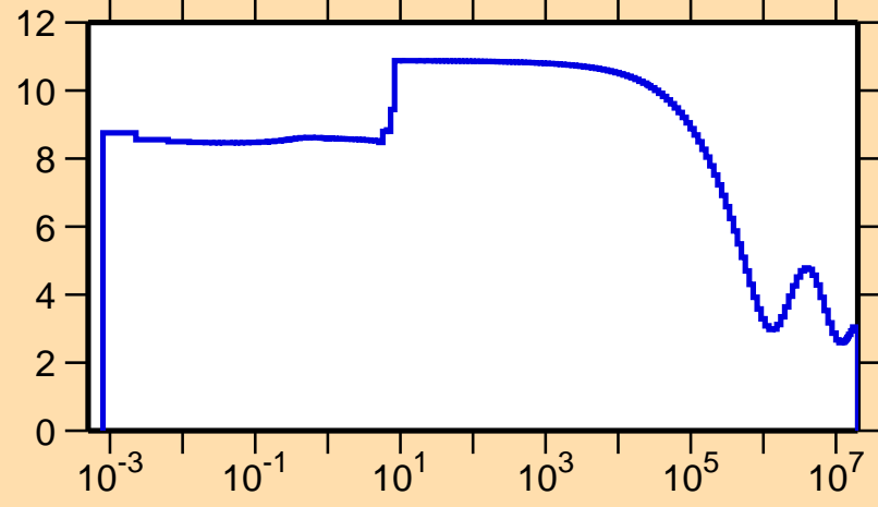
\sigma vs. E for ^{234}\text{Am}(n,\text{el.})
