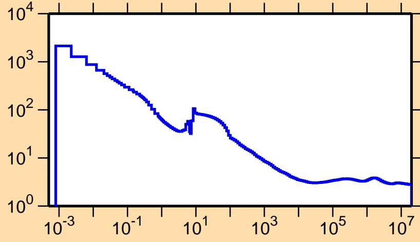
\sigma vs. E for ^{234}\text{Am}(n,f)
