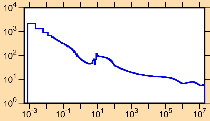
\sigma vs. E for ^{234}\text{Am}(n,\text{tot.})
