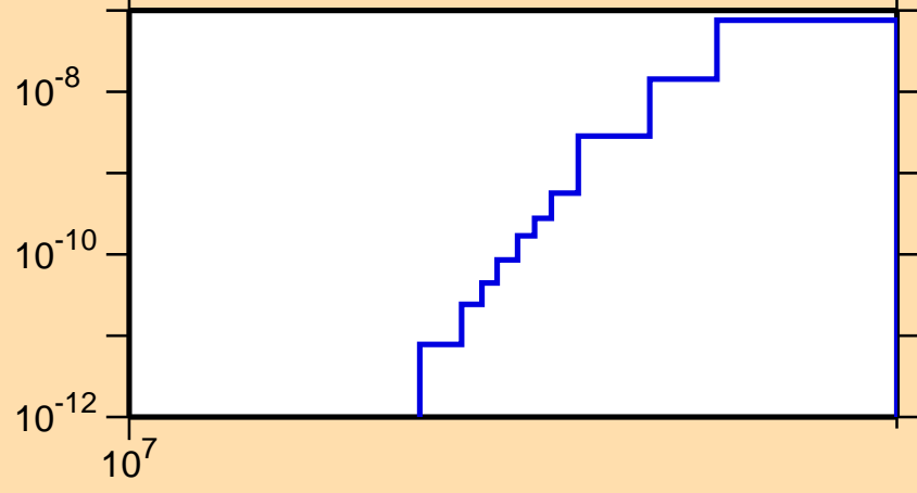
\sigma vs. E for ^{234}\text{Am}(n,\text{nd})
