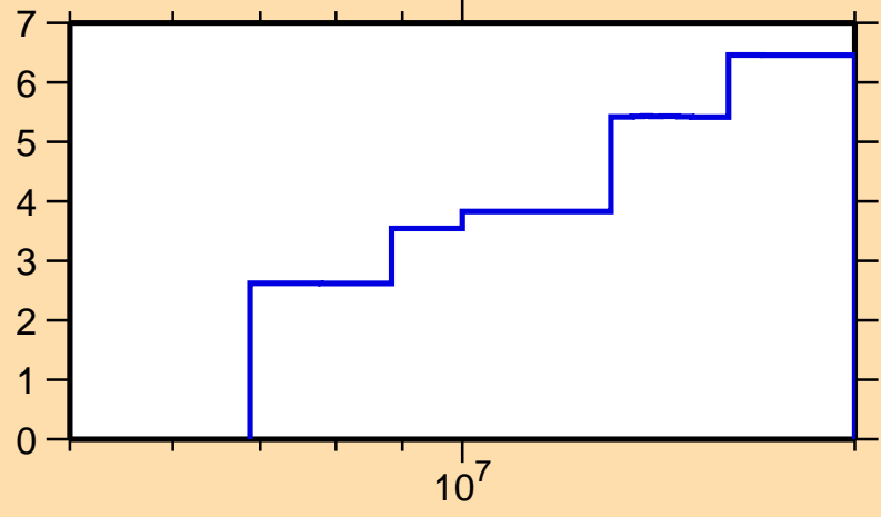
\Delta\sigma/\sigma vs. E for ^{234}\text{Am}(n,\text{nonel.})
