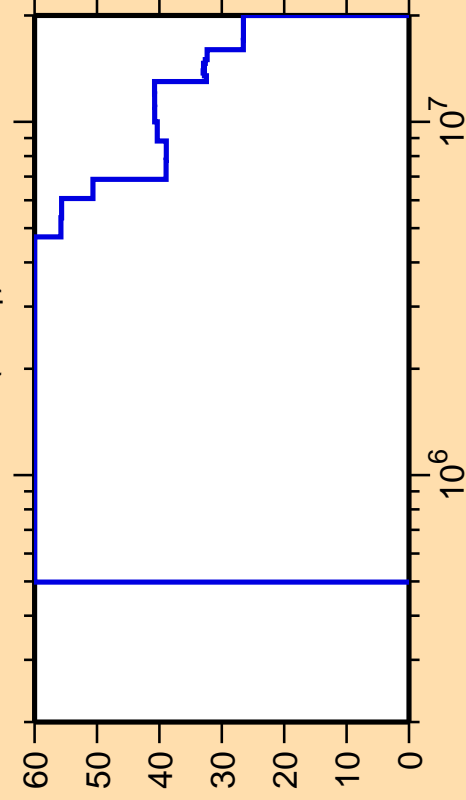
\Delta\sigma/\sigma vs. E for ^{234}\text{Am}(n,n_1)
