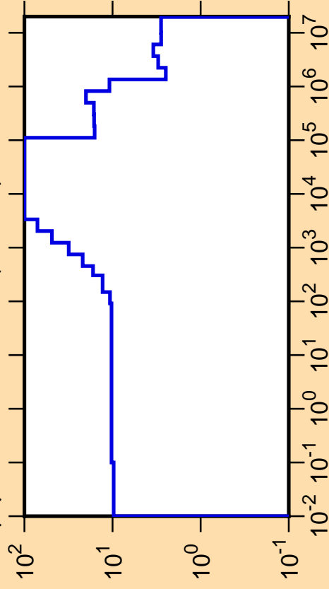
\Delta\mu/\mu vs. E for ^{234}\text{Am}(\text{mt251})
