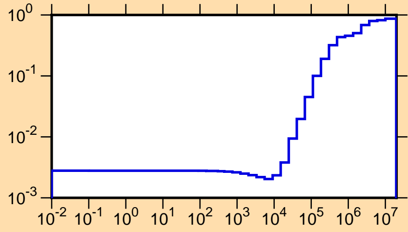
\mu vs. E for ^{234}\text{Am}(\text{mt251})
