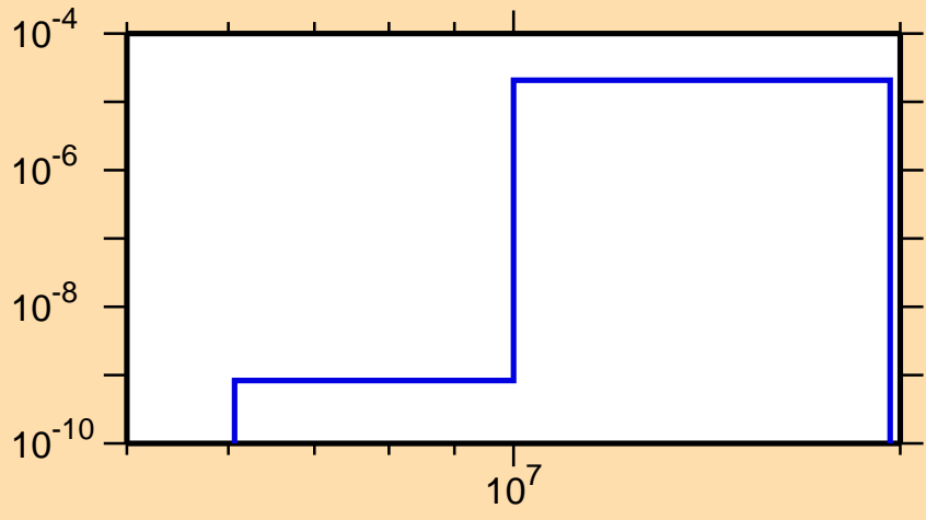
\sigma vs. E for ^{234}\text{Am}(n,np)
