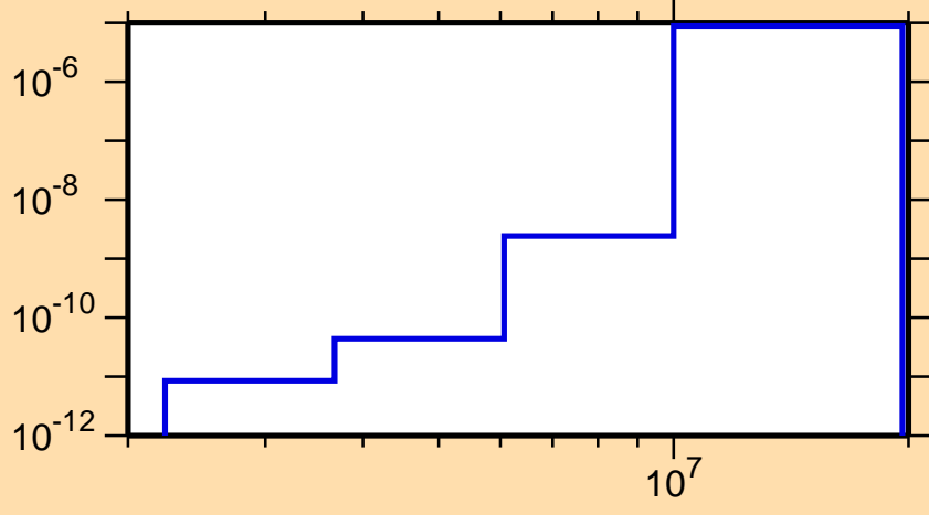
\sigma vs. E for ^{234}\text{Am}(n,n\alpha)
