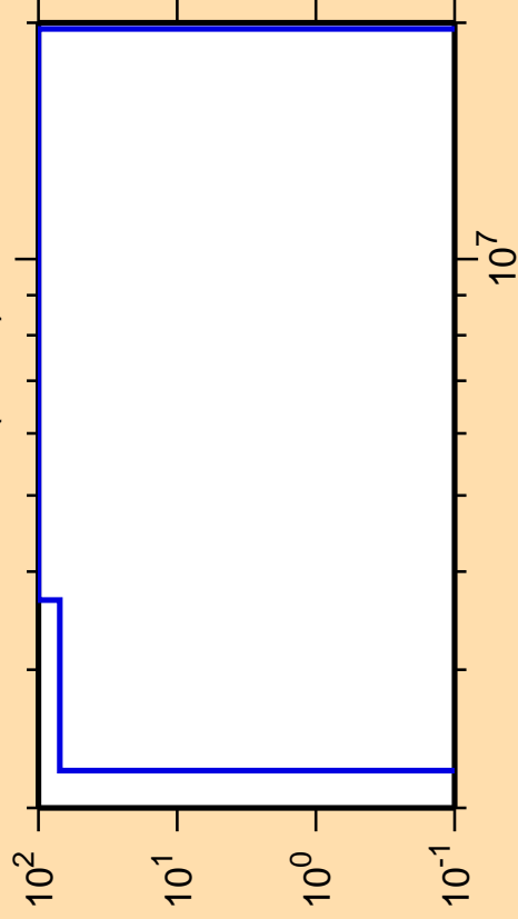
\Delta\sigma/\sigma vs. E for ^{234}\text{Am}(n,n\alpha)
