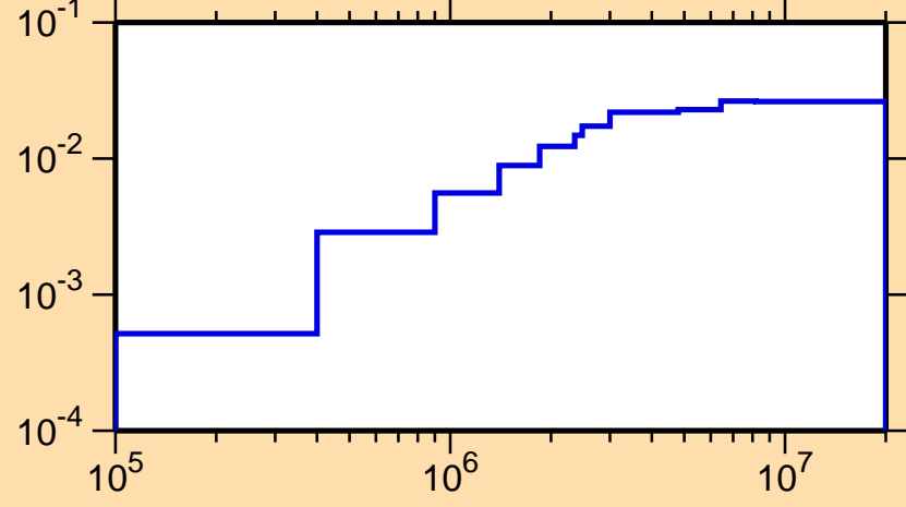
\sigma vs. E for ^{234}\text{Am}(n,\text{inel.})
