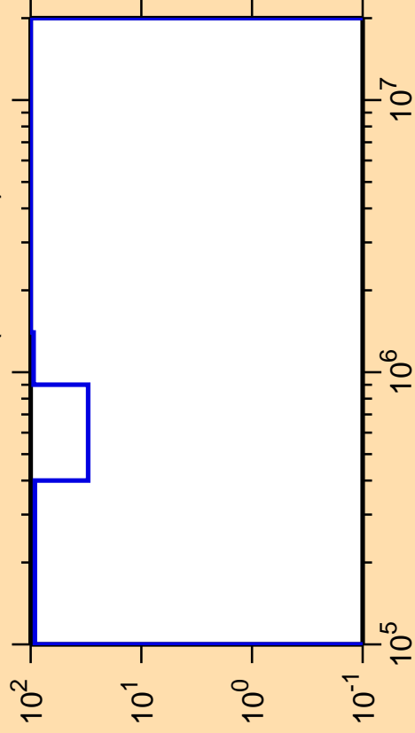
\Delta\sigma/\sigma vs. E for ^{234}\text{Am}(n,\text{ncont.})
