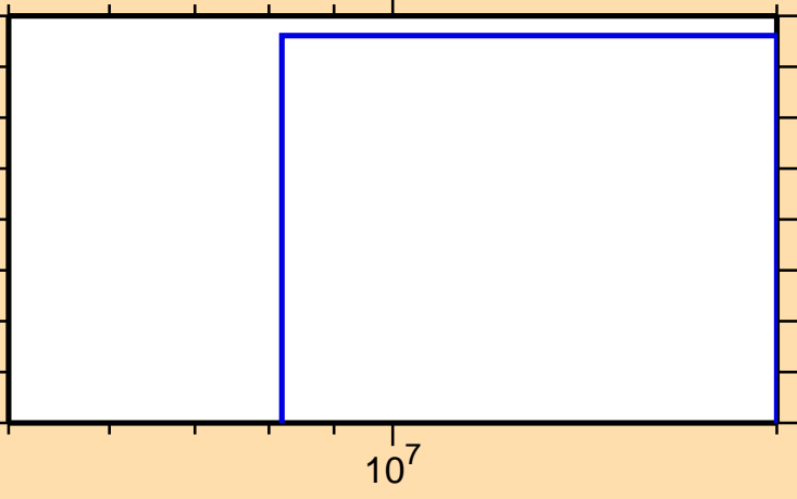
\sigma vs. E for ^{234}\text{Am}(n,2np)
