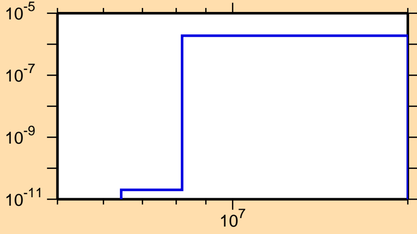
\sigma vs. E for ^{234}\text{Am}(n,t)
