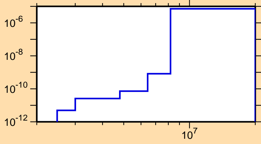
\sigma vs. E for ^{234}\text{Am}(n,\alpha)
