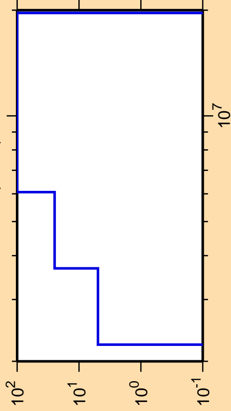
\Delta\sigma/\sigma vs. E for ^{235}\text{Am}(n,n\alpha)
