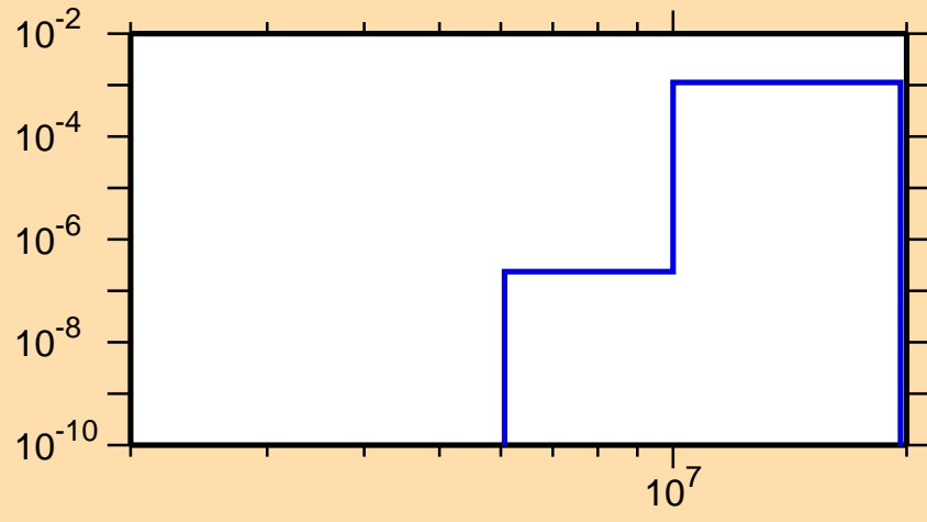
\sigma vs. E for ^{235}\text{Am}(n,d)
