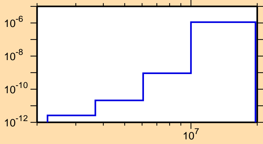
\sigma vs. E for ^{235}\text{Am}(n,n\alpha)
