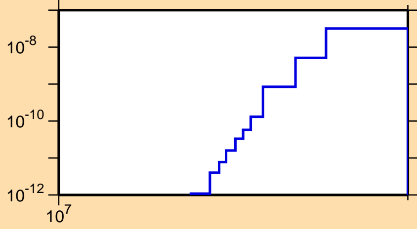
\sigma vs. E for ^{236}\text{Am}(n,nd)
