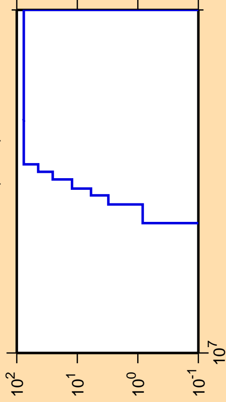
\Delta\sigma/\sigma vs. E for ^{236}\text{Am}(n,nd)
