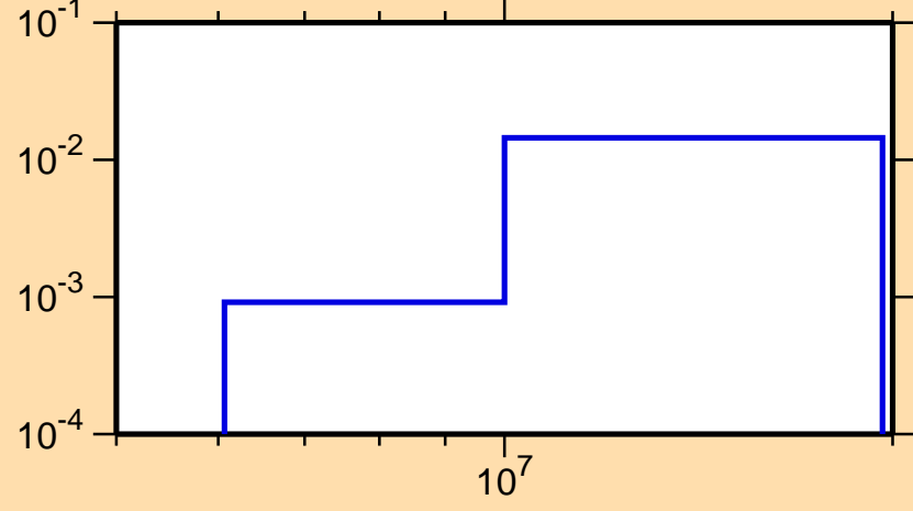
\sigma vs. E for ^{236}\text{Am}(n,2n)
