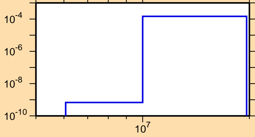
\sigma vs. E for ^{236}\text{Am}(n,t)
