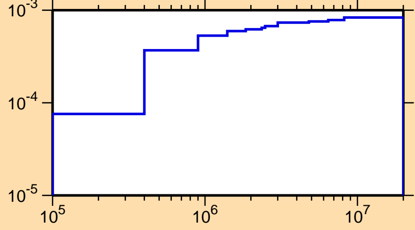
\sigma vs. E for ^{236}\text{Am}(n,n_1)
