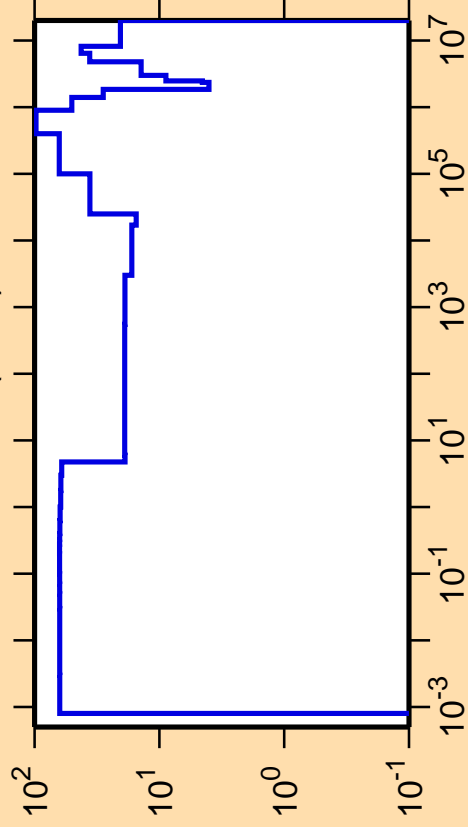
\Delta\sigma/\sigma vs. E for ^{236}\text{Am}(n,\text{el.})
