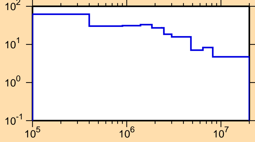
\Delta\sigma/\sigma vs. E for ^{236}\text{Am}(n,\text{nonel.})
