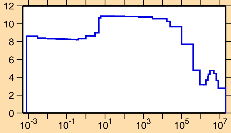
\sigma vs. E for ^{236}\text{Am}(n,\text{el.})
