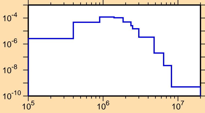
\sigma vs. E for ^{236}\text{Am}(n,n_4)
