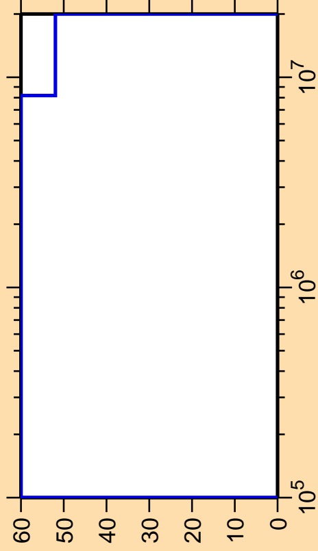
\Delta\sigma/\sigma vs. E for ^{236}\text{Am}(n,n_4)
