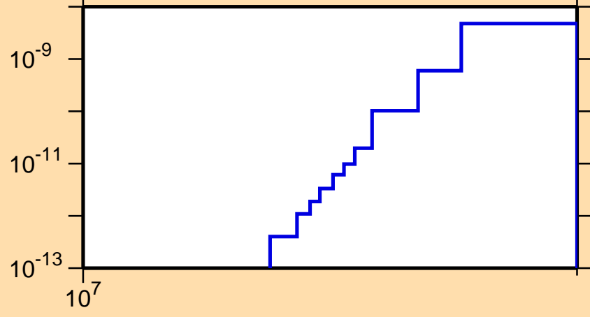
\sigma vs. E for ^{237}\text{Am}(n,\text{He3})
