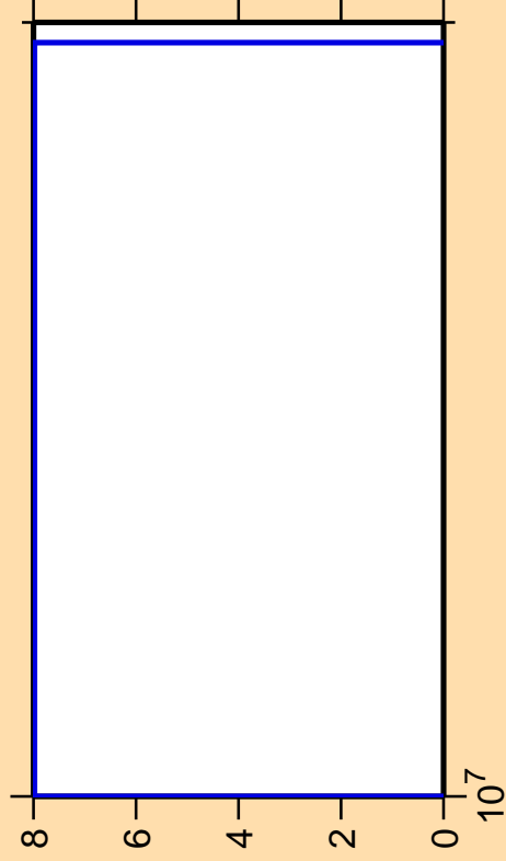
\Delta\sigma/\sigma vs. E for ^{237}\text{Am}(n,p\alpha)
