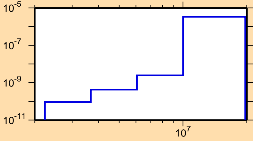
\sigma vs. E for ^{237}\text{Am}(n,\alpha)
