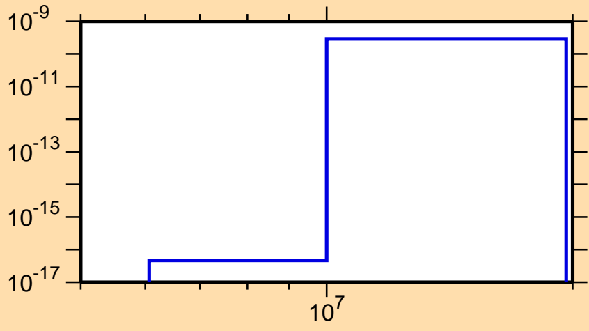
\sigma vs. E for ^{237}\text{Am}(n,2n\alpha)
