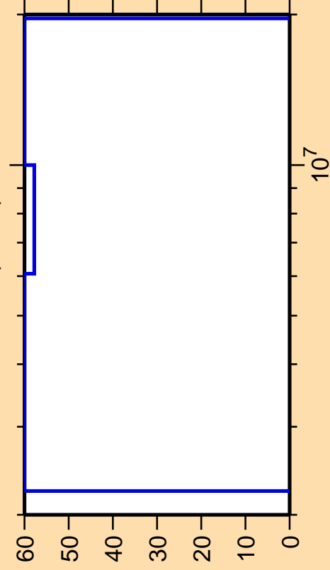
\Delta\sigma/\sigma vs. E for ^{237}\text{Am}(n,\alpha)
