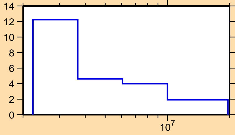
\Delta\sigma/\sigma vs. E for ^{237}\text{Am}(n,n\text{onel.})
