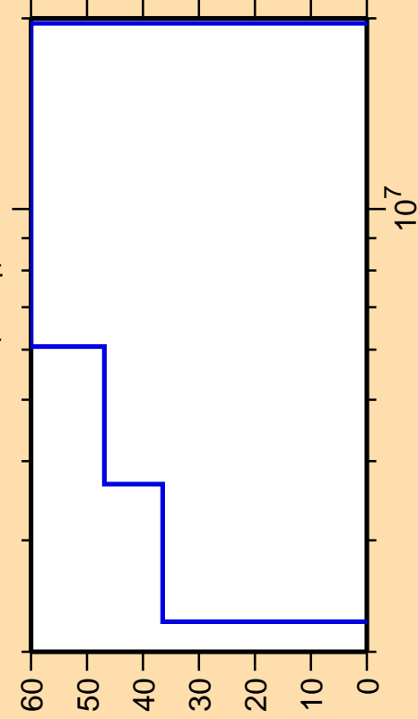
\Delta\sigma/\sigma vs. E for ^{237}\text{Am}(n,n_1)
