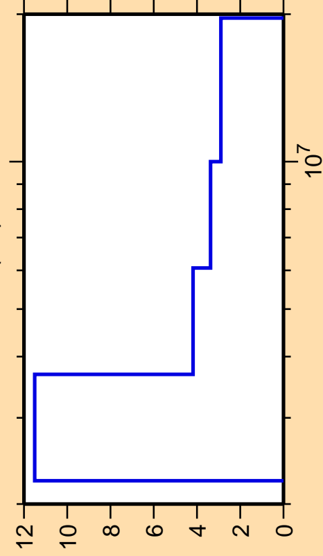
\Delta\sigma/\sigma vs. E for ^{237}\text{Am}(n,f)
