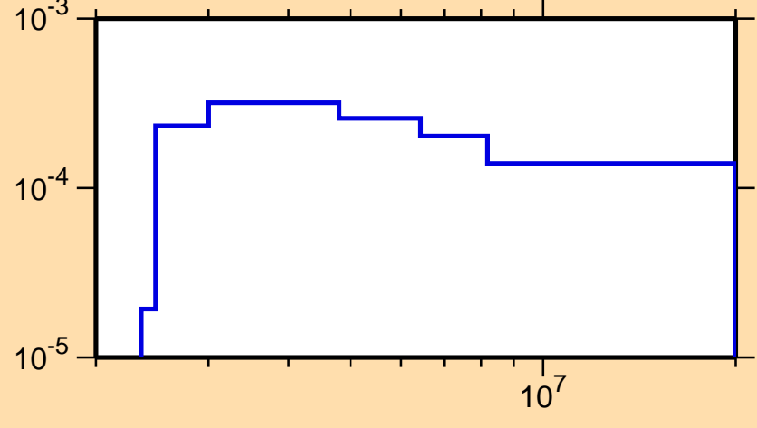
\sigma vs. E for ^{237}\text{Am}(n,n_1)
