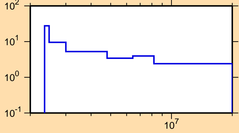
\Delta\sigma/\sigma vs. E for ^{237}\text{Am}(n,f)
