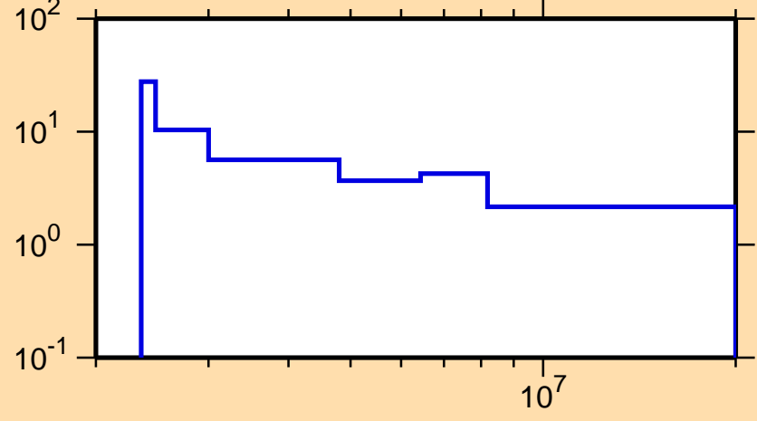
\Delta\sigma/\sigma vs. E for ^{237}\text{Am}(n,\text{nonel.})
