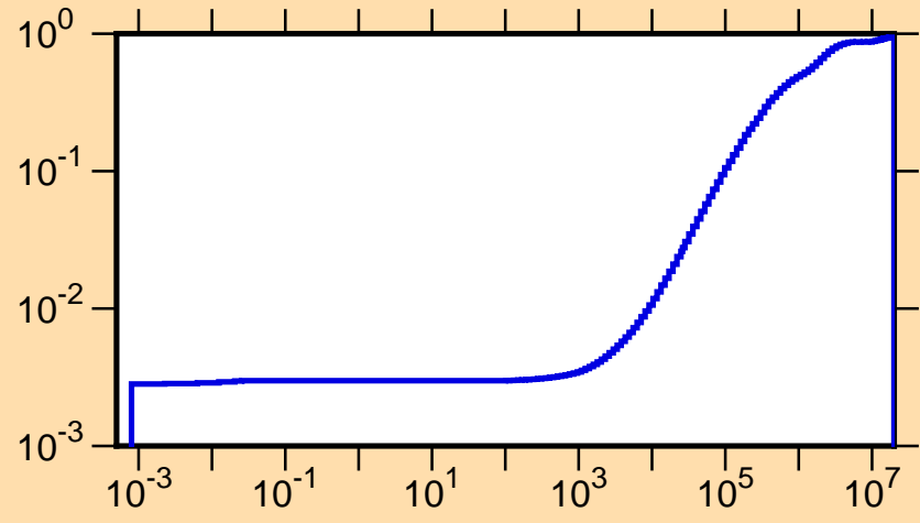
\mu vs. E for ^{239}\text{Am}(\text{mt251})
