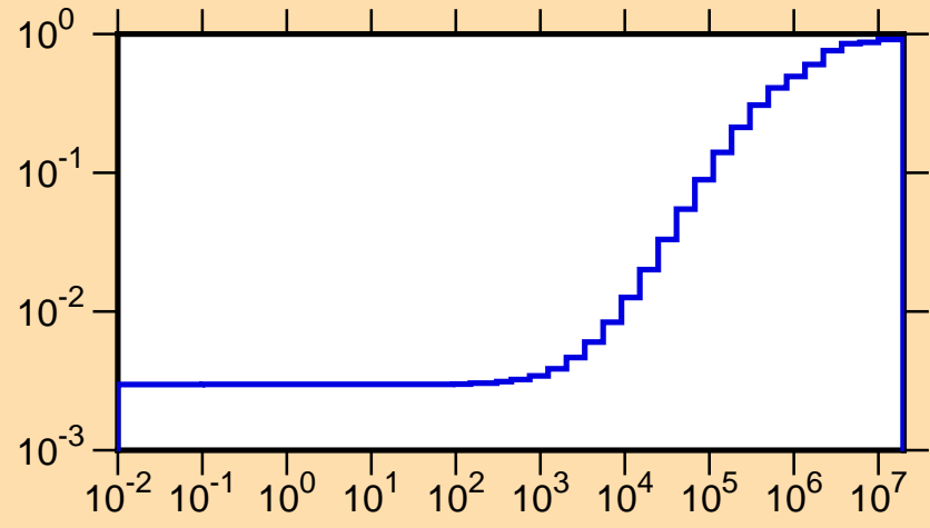
\mu vs. E for ^{239}\text{Am} (mt251)
