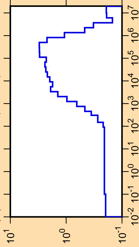
\Delta\mu/\mu vs. E for ^{239}\text{Am} (mt251)
