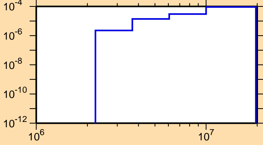
\sigma vs. E for ^{239}\text{Am}(n,\alpha)
