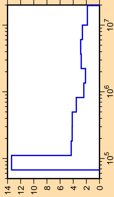
\Delta\sigma/\sigma vs. E for ^{239}\text{Am}(n,n_2)
