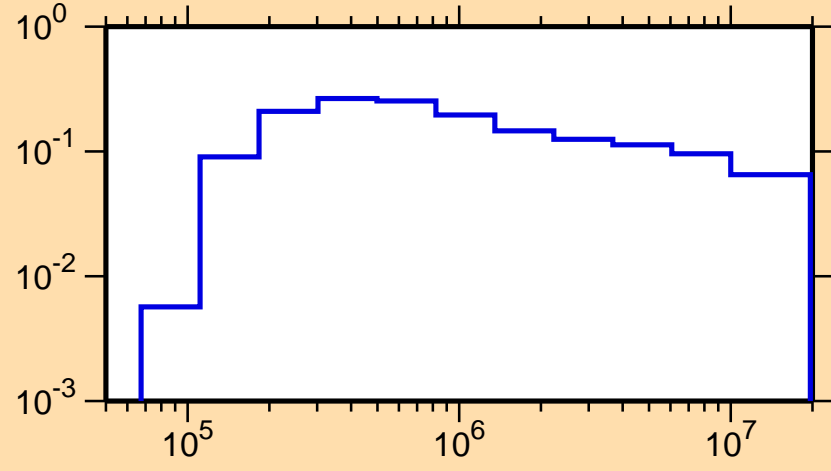
\sigma vs. E for ^{239}\text{Am}(n,n_2)
