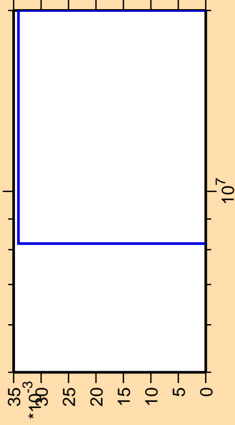
\Delta\sigma/\sigma vs. E for ^{239}\text{Am}(n,3n\alpha)
