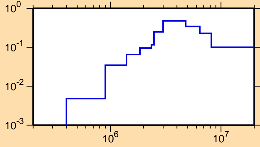
\sigma vs. E for ^{239}\text{Am}(n,n\text{cont.})
