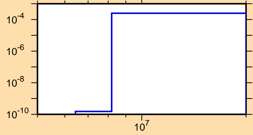
\sigma vs. E for ^{239}\text{Am}(n,np)
