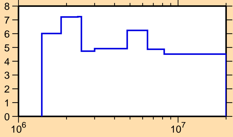
\Delta\sigma/\sigma vs. E for ^{239}\text{Am}(n,ncont.)
