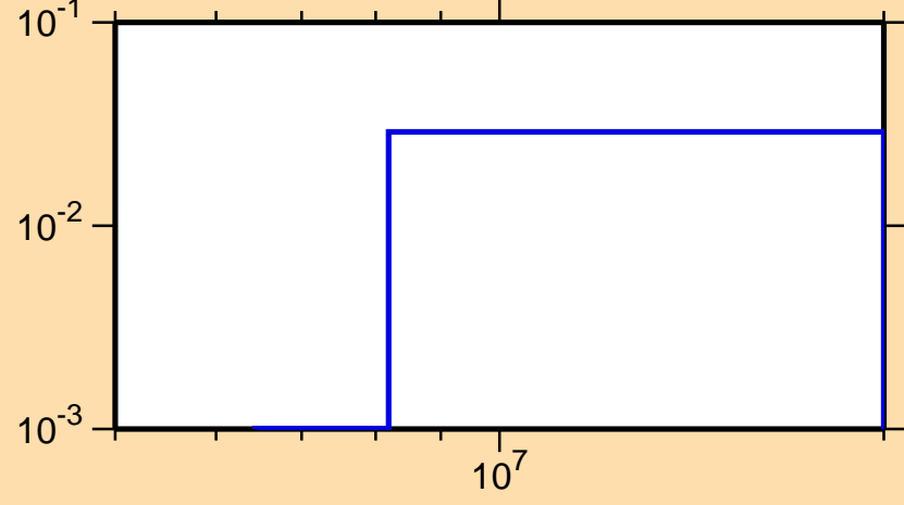
\sigma vs. E for ^{239}\text{Am}(n,2n)
