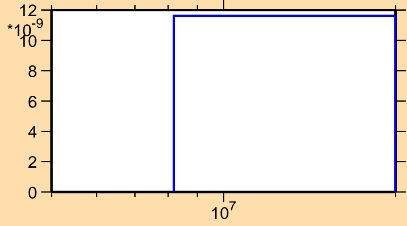
\sigma vs. E for ^{239}\text{Am}(n,\text{nd})
