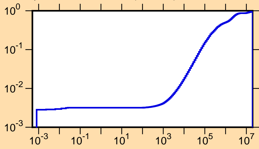
\mu vs. E for ^{240}\text{Am}(\text{mt251})
