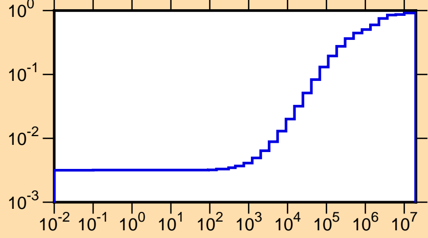
\mu vs. E for ^{240}\text{Am}(\text{mt251})
