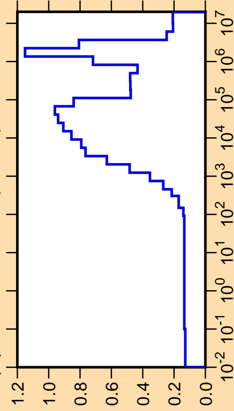
\Delta\mu/\mu vs. E for ^{240}\text{Am}(\text{mt251})
