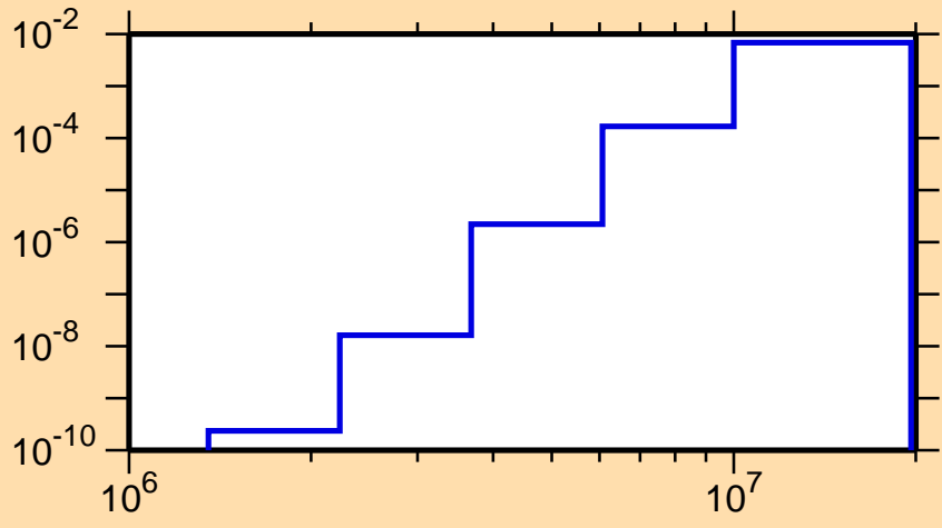
\sigma vs. E for ^{240}\text{Am}(n,p)
