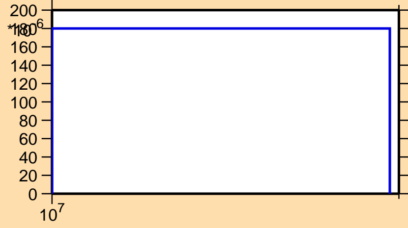
\sigma vs. E for ^{240}\text{Am}(n,3n)
