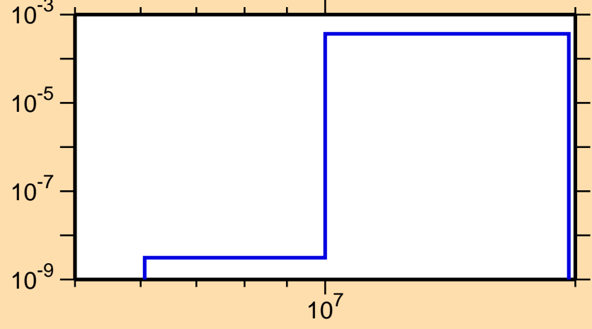
\sigma vs. E for ^{240}\text{Am}(n,d)
