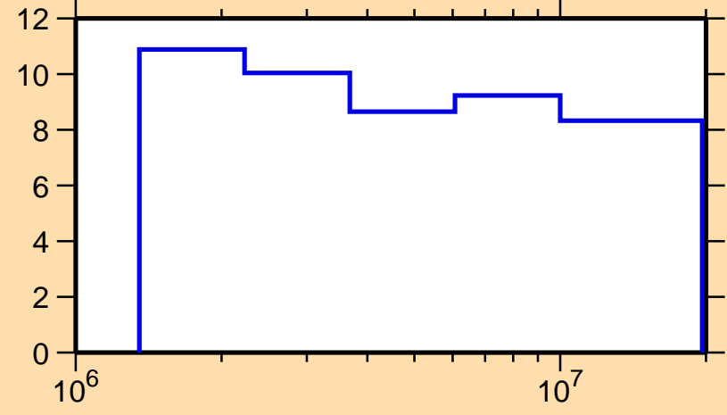
\Delta\sigma/\sigma vs. E for ^{240}\text{Am}(n,n\text{cont.})
