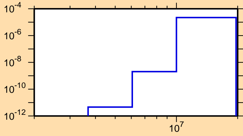
\sigma vs. E for ^{240}\text{Am}(n,n\alpha)
