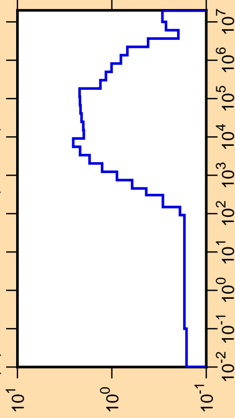
\Delta\mu/\mu vs. E for ^{241}\text{Am}(\text{mt251})
