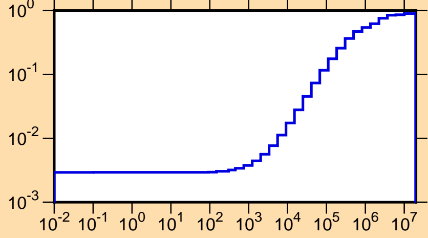
\mu vs. E for ^{241}\text{Am}(\text{mt251})
