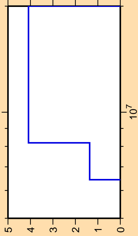
\Delta\sigma/\sigma vs. E for ^{241}\text{Am}(n,np)
