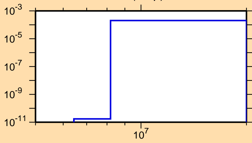
\sigma vs. E for ^{241}\text{Am}(n,np)
