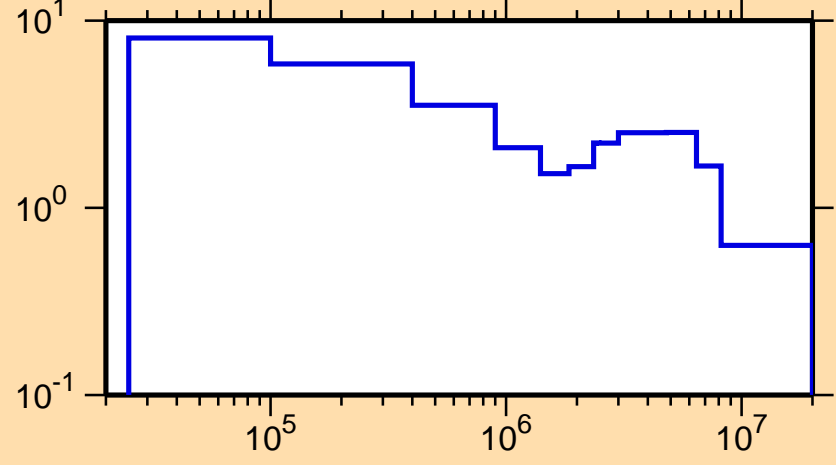
\Delta\sigma/\sigma vs. E for ^{241}\text{Am}(n,\text{nonel.})
