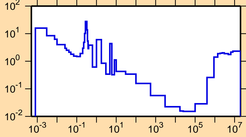
\sigma vs. E for ^{241}\text{Am}(n,f)
