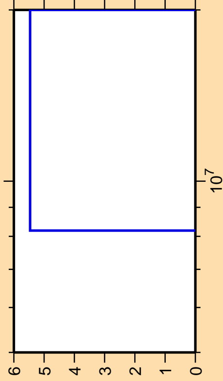
\Delta\sigma/\sigma vs. E for ^{241}\text{Am}(n,3n)
