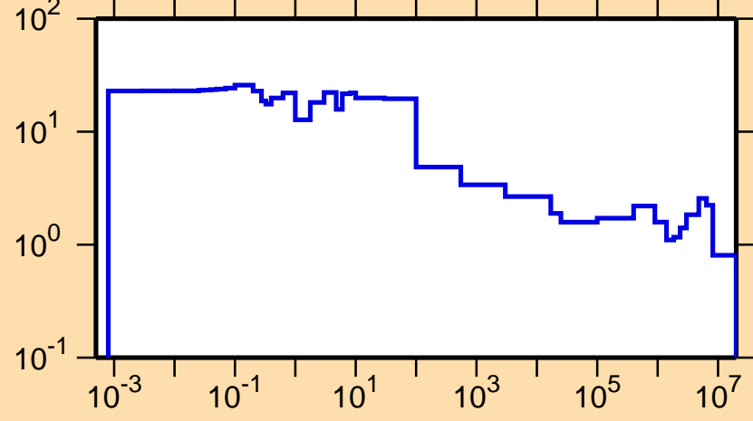
\Delta\sigma/\sigma vs. E for ^{241}\text{Am}(n,el.)
