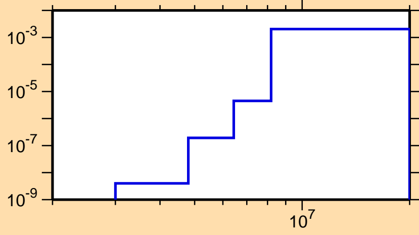
\sigma vs. E for ^{241}\text{Am}(n,p)
