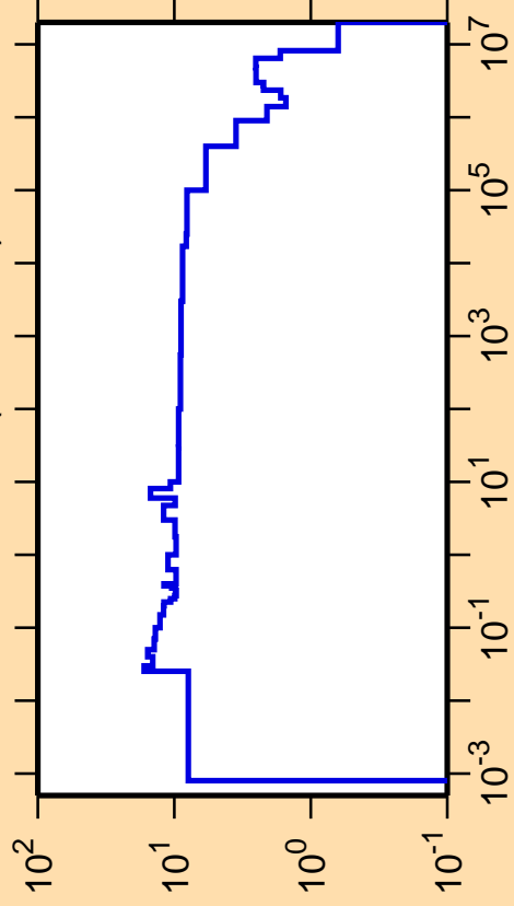
\Delta\sigma/\sigma vs. E for ^{241}\text{Am}(n,\text{nonel.})
