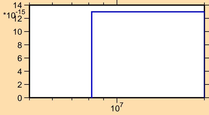
\sigma vs. E for ^{241}\text{Am}(\text{mt } 11)
