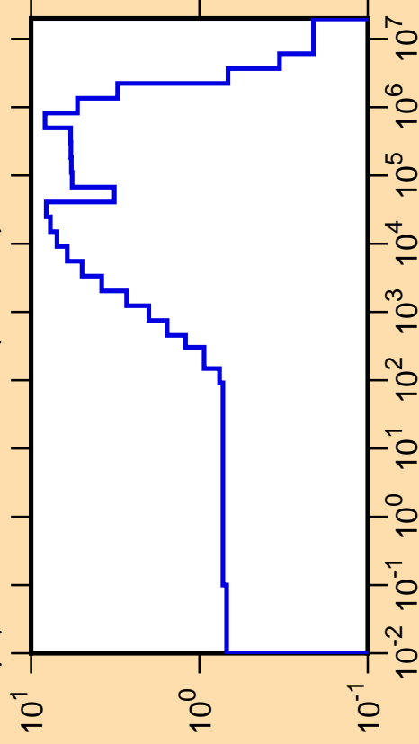
\Delta\mu/\mu vs. E for ^{242}\text{Am}(\text{mt251})
