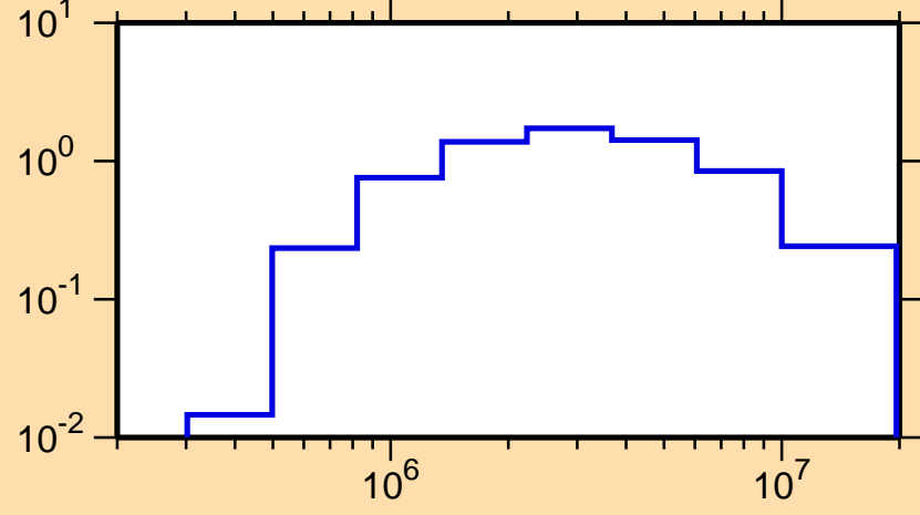
\sigma vs. E for ^{242}\text{Am}(n,n\text{cont.})
