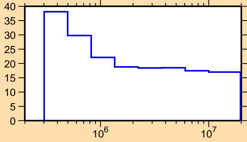
\Delta\sigma/\sigma vs. E for ^{242}\text{Am}(n, ncont.)
