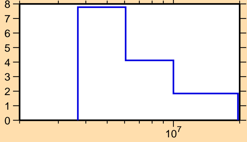
\Delta\sigma/\sigma vs. E for ^{242}\text{Am}(n,\text{nonel.})
