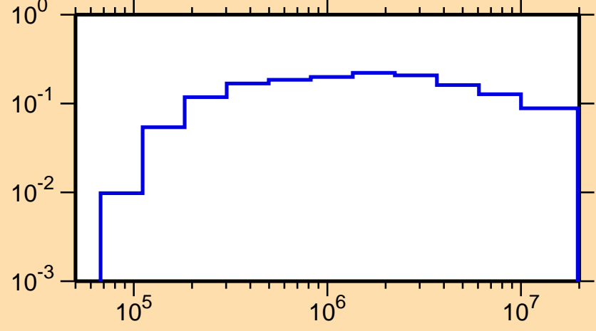
\sigma vs. E for ^{242}\text{Am}(n,n_4)
