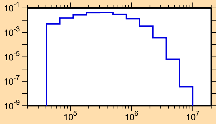
\sigma vs. E for ^{242}\text{Am}(n,n_1)
