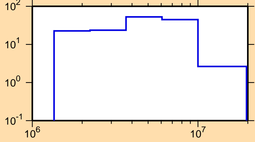
\Delta\sigma/\sigma vs. E for ^{242}\text{Am}(n,n_1)
